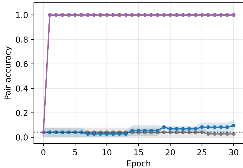
A. Fingerprint emerges only under adaptive optimizers
