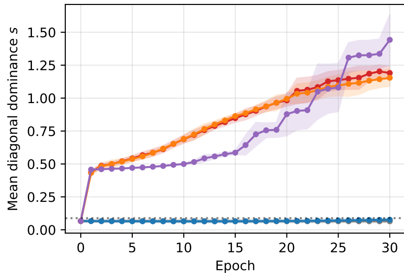
B. Diagonal structure climbs only with Adam/AdamW/RMSprop
