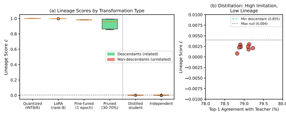
Figure 6: GPT-2-Small-Lite lineage benchmark (8 roots, 120 pairs). (a) Lineage scores by transformation type. Descendants (green) score high; non-descendants (red) score near zero. (b) Distilled students achieve high behavioral agreement (79% top-1) yet score far below the minimum descendant threshold, confirming that imitation \neq inheritance.
