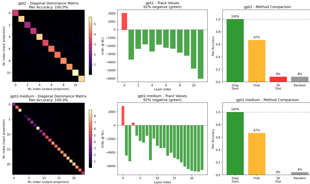
Figure 13. GPT-2 MLP pairing results. Left column: diagonal-dominance matrices showing bright diagonals (correct pairs). Center: trace values per layer; green bars indicate negative traces consistent with dynamic isometry. Right: method comparison showing diagonal dominance dramatically outperforms Frobenius and SV-distance baselines.
