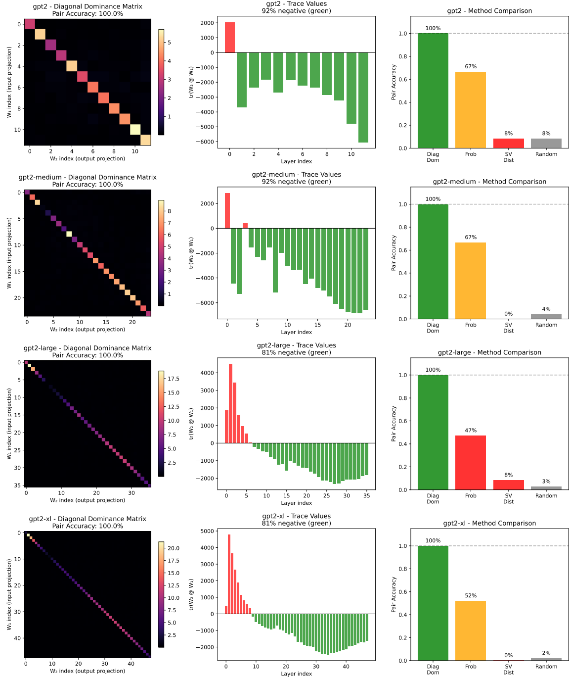
Figure 5: GPT-2 MLP pairing results. Left: Diagonal-dominance matrices for GPT-2 (124M, 12 layers) and GPT-2-XL (1.5B, 48 layers)—bright diagonals indicate perfect pairing. Center: Trace values per layer; 81–92% are negative, consistent with dynamical isometry. Right: Method comparison showing diagonal-dominance achieves 100% accuracy while Frobenius matching plateaus at 47–67%.
