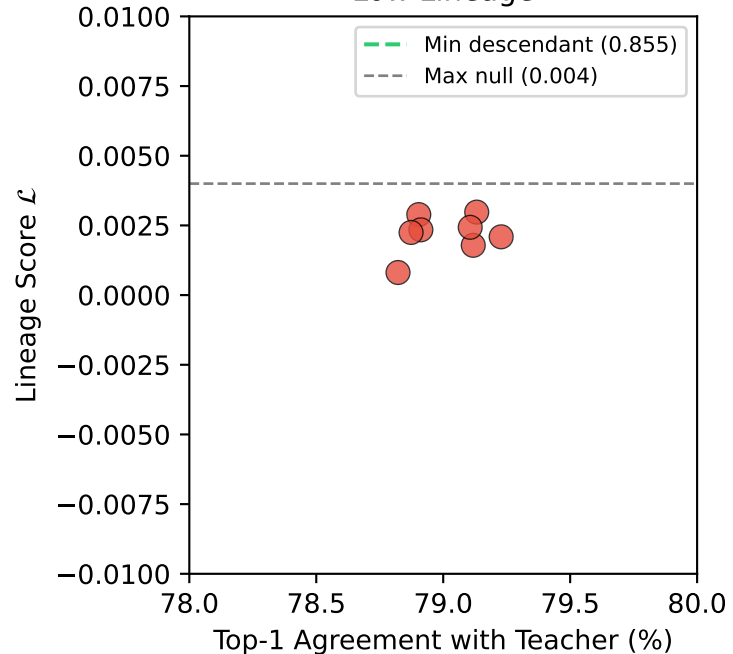
(b) Distillation: High Imitation, Low Lineage
