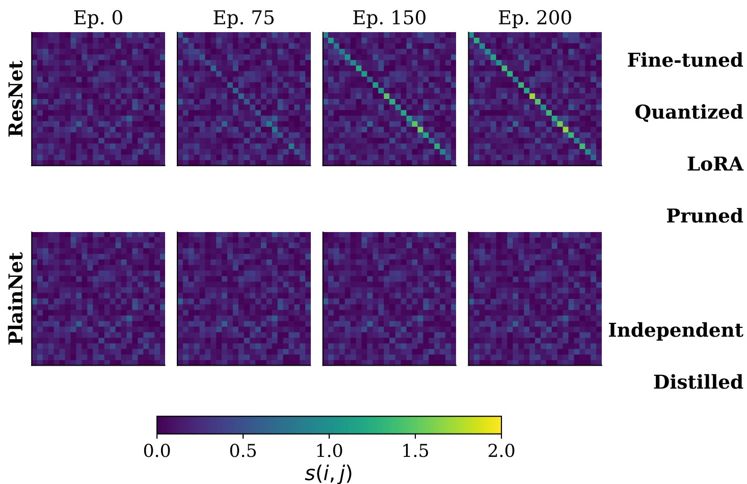
(b) Training Induces Diagonal Dominance: ResNet vs PlainNet
