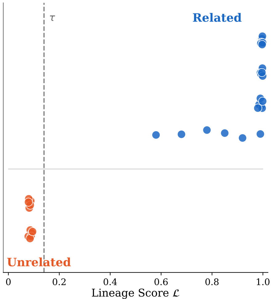
(c) White-Box Model Lineage Verification
