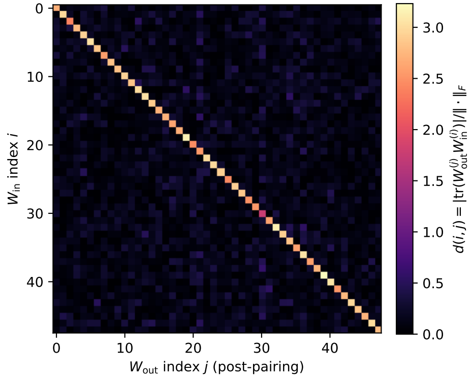
(b) Trained ResNet (Park's puzzle, recovered pairing) pair acc = 1.00, sep = +1.36
