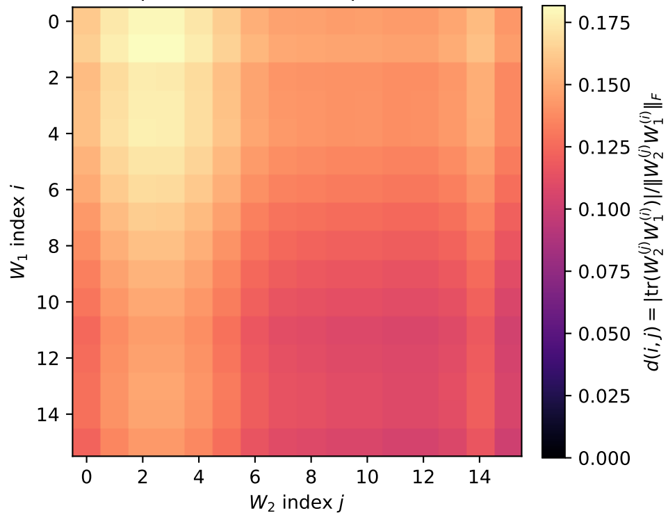
(b) Trained transformer MLPs pair acc = 0.00, sep = -0.04
