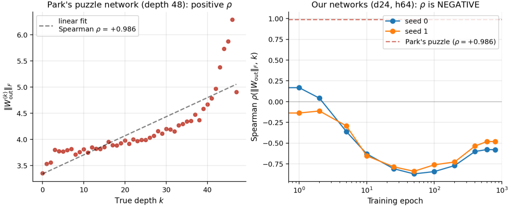
Figure 10. Spearman correlation of \|W_{\text{out}}\|_F with true depth. Left: Park’s puzzle network has \rho = +0.986 . Right: our 24-block synthetic ResNets across training, two seeds. \rho is negative throughout, reaching -0.87 mid-training and weakening with continued optimization.
