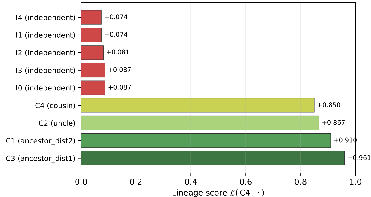
Ancestry ranking for C4
