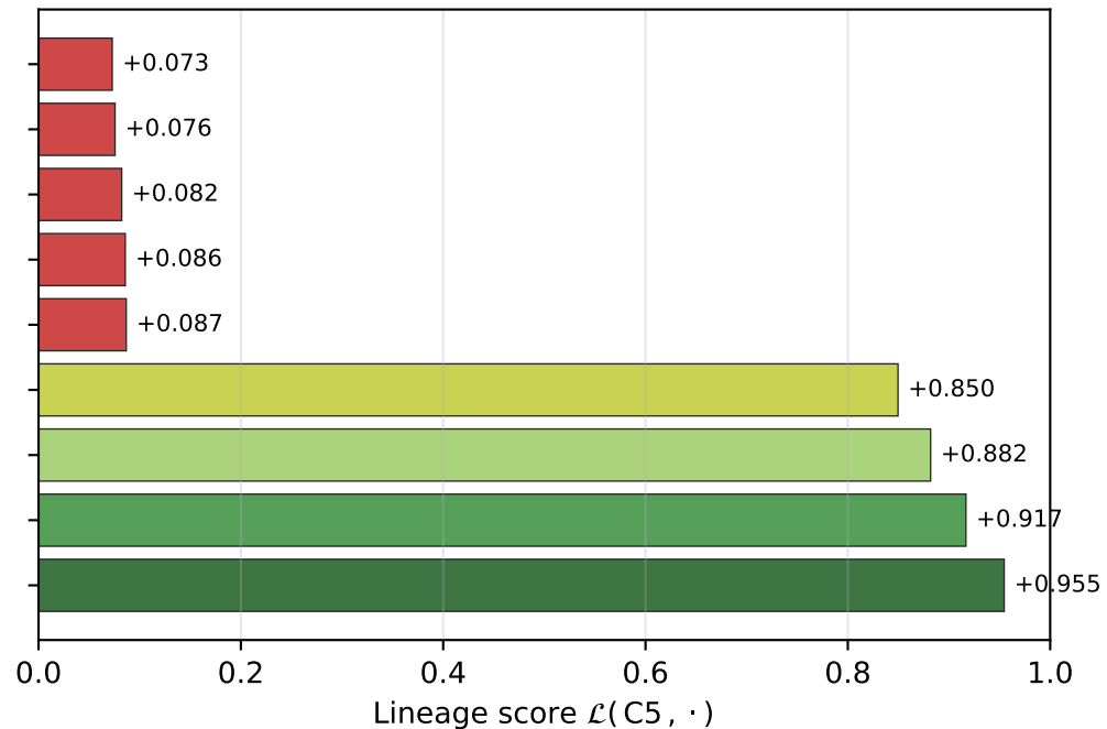
Ancestry ranking for C5
