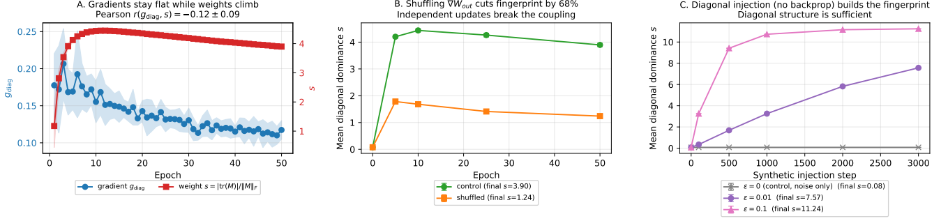
Figure 2: The fingerprint is a causal product of gradient coupling between W_{in} and W_{out} . (a) The gradient product itself does not become diagonal, so the mechanism couples update directions, not diagonal shape. (b) Necessity: shuffling \nabla W_{out} across blocks drops the score by 68% while training proceeds. (c) Sufficiency: direct diagonal injection builds the score with no backpropagation.
