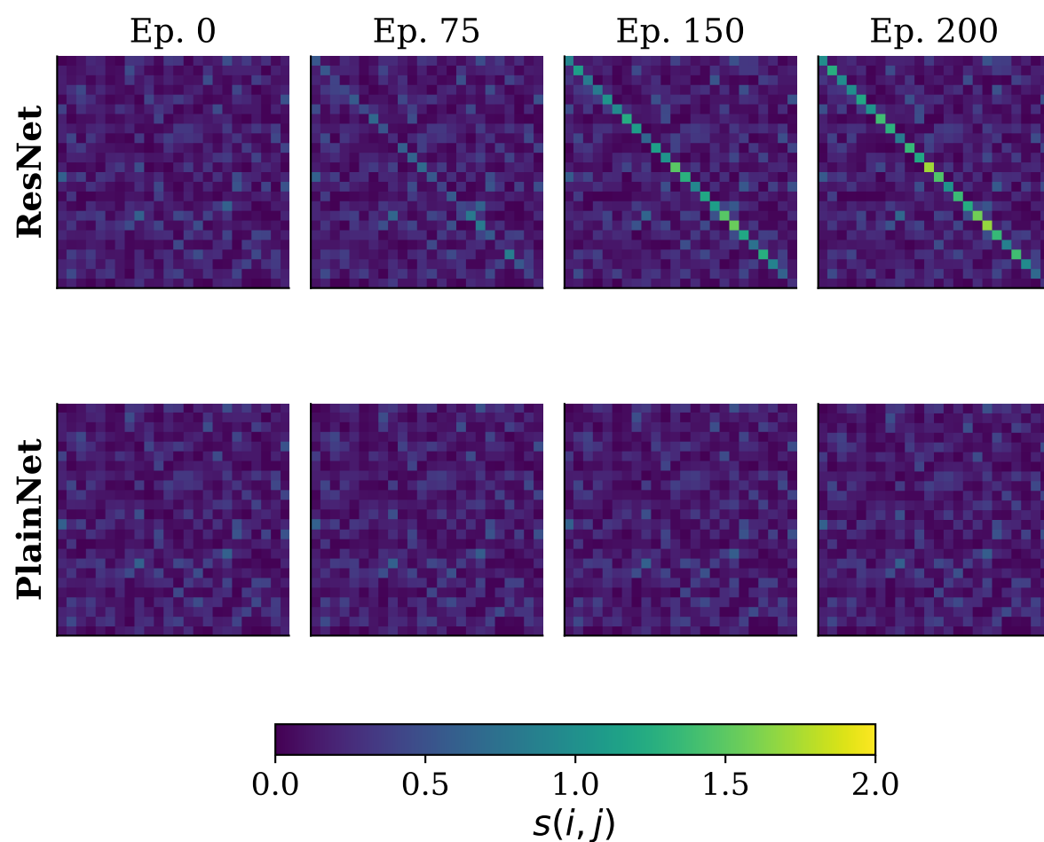
(b) Training Induces Diagonal Dominance: ResNet vs PlainNet
