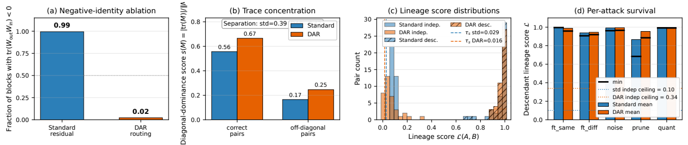
Figure 6: Fingerprint survives DAR cross-layer routing on depth-24 MLPs at matched plateau. (a) Negative-identity component is ablated under DAR ( 0.99 \rightarrow 0.02 ). (b) Trace concentration on correct pairs is preserved; separation from off-diagonal pairs is comparable to standard residual. (c) Lineage score distributions remain bimodal with AUROC=1.000 for both architectures. (d) Per-attack descendant scores stay above each architecture’s independent ceiling across noise, pruning, quantization, and same/different-target fine-tuning.
