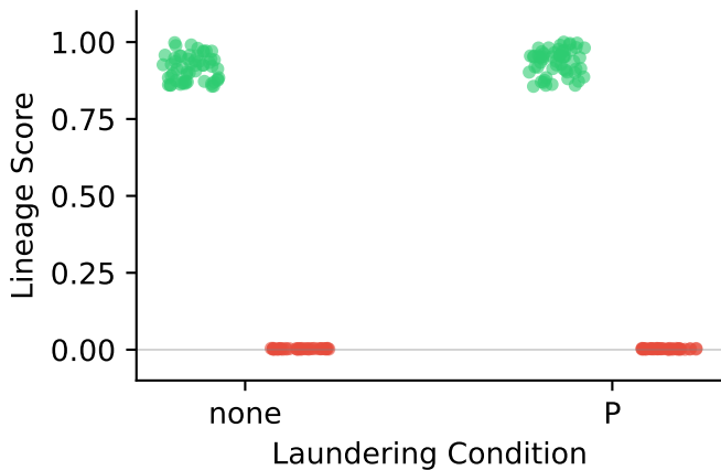
(c) GPT-2: Ours
