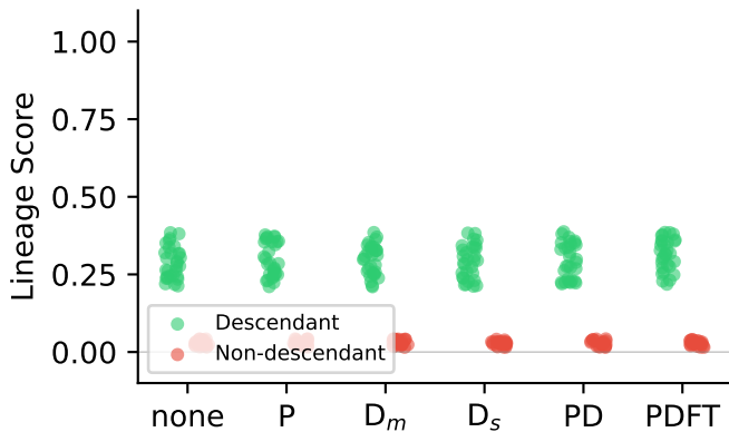
(c) GPT-2: Ours
