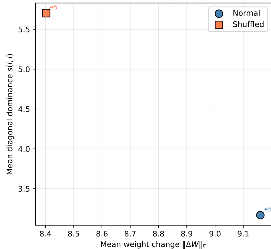
P0.5 Control: s vs Weight Magnitude
