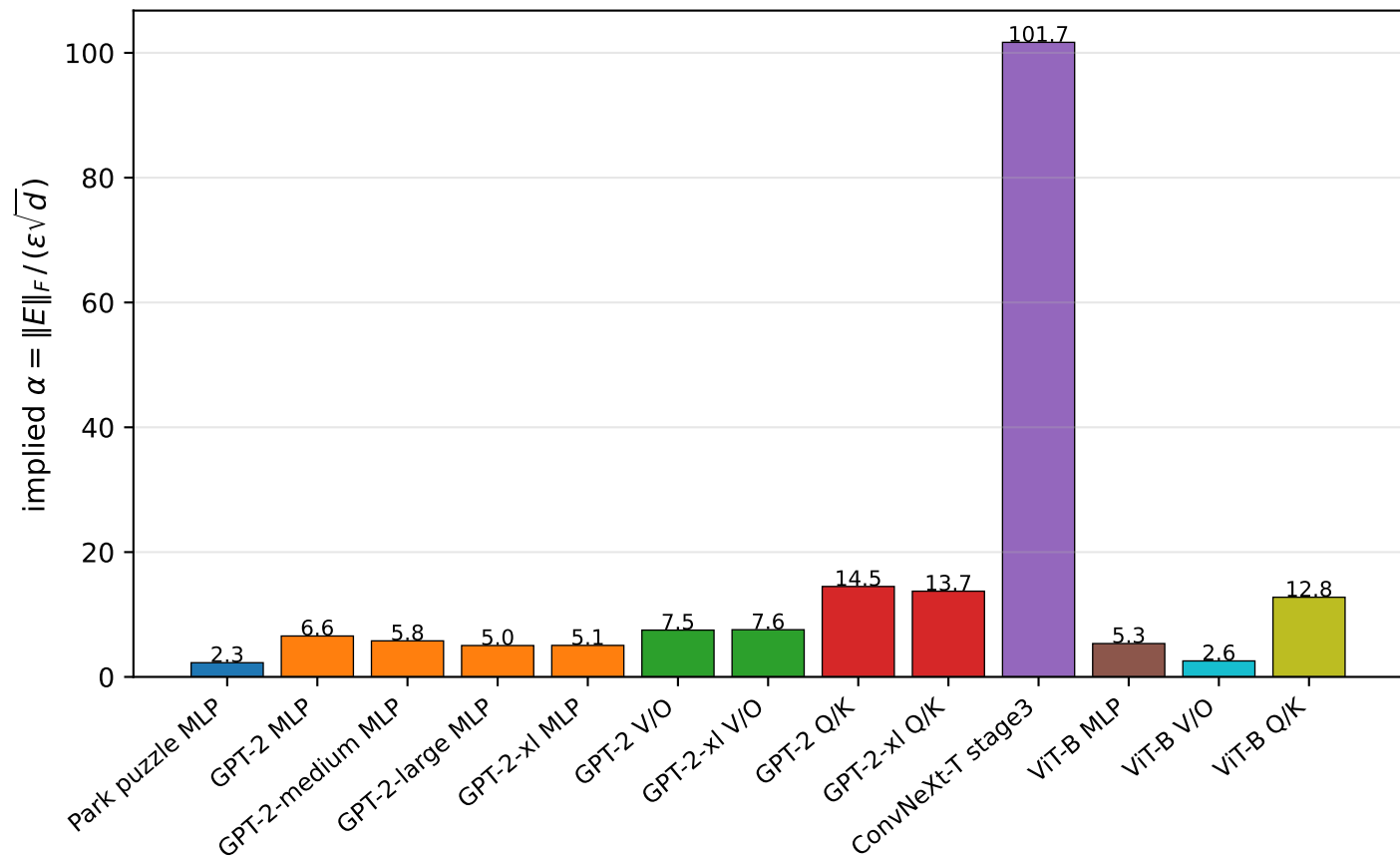
(b) Off-diagonal energy relative to scaled identity (lower = closer to -\epsilon I )
