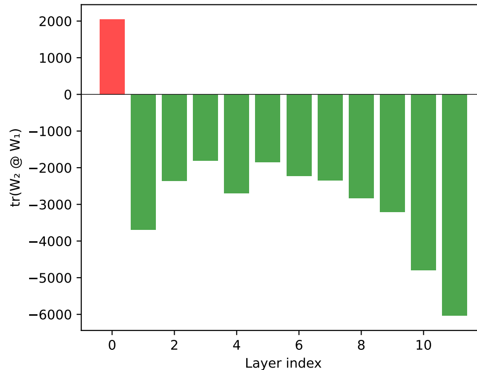
gpt2 - Trace Values 92% negative (green)
