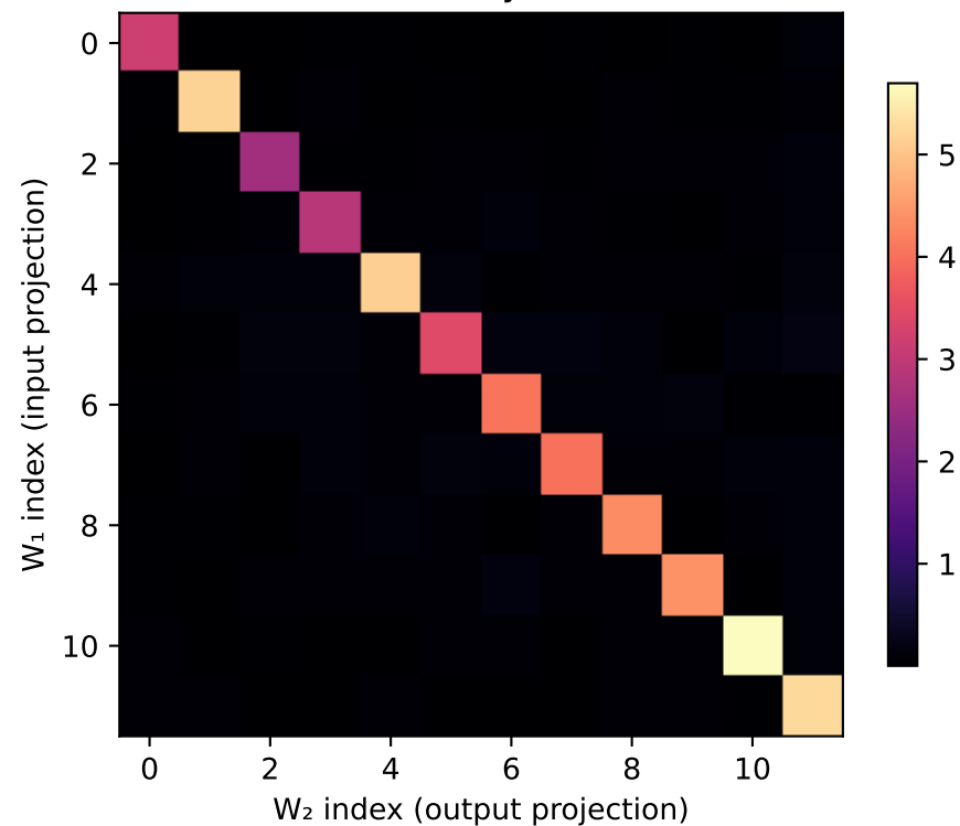
gpt2 - Diagonal Dominance Matrix Pair Accuracy: 100.0%
