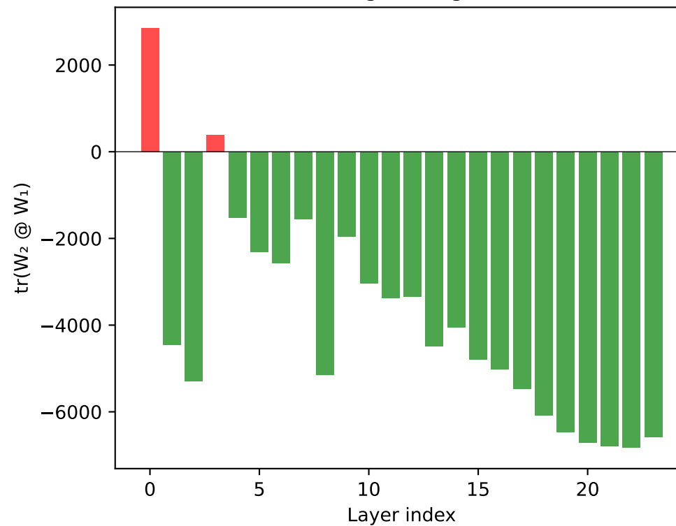
gpt2-medium - Trace Values 92% negative (green)
