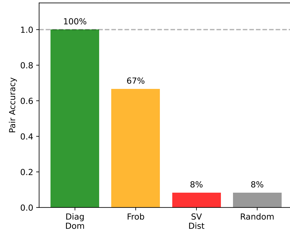
gpt2 - Method Comparison
