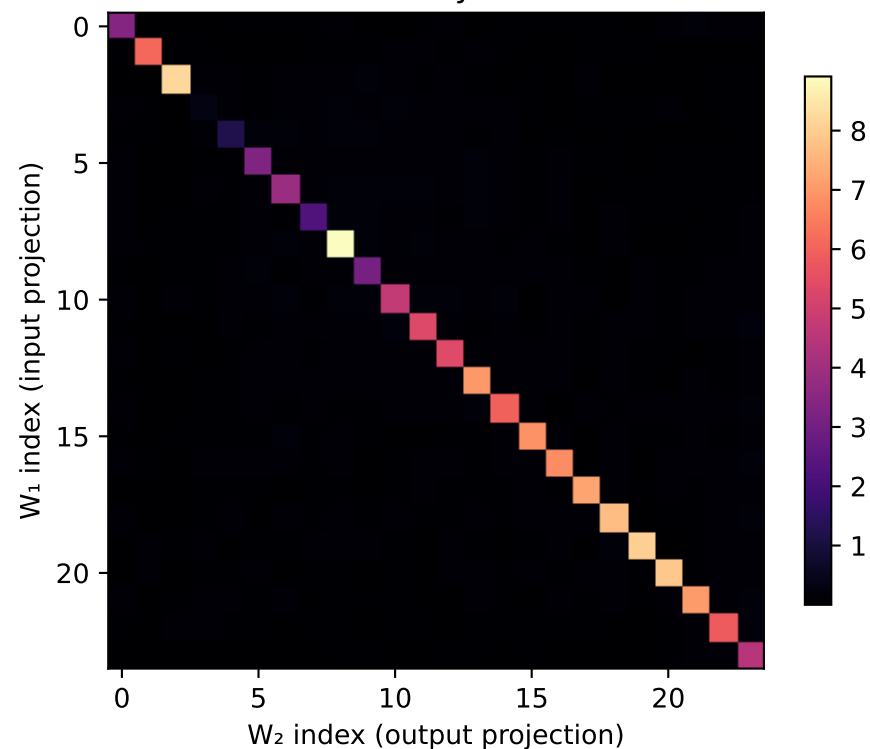
gpt2-medium - Diagonal Dominance Matrix Pair Accuracy: 100.0%
