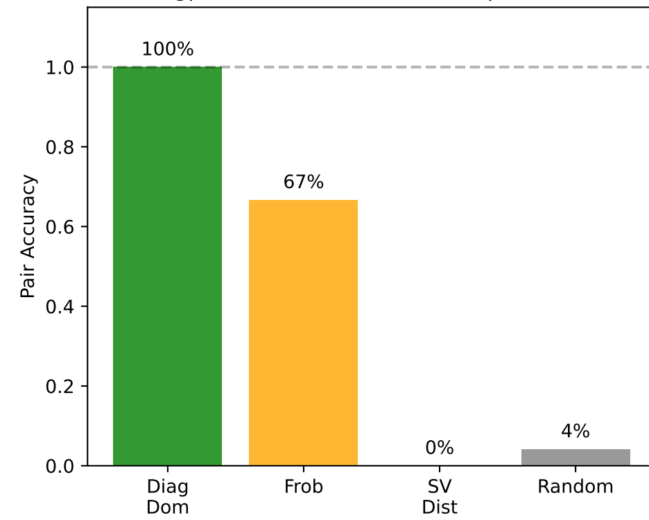
gpt2-medium - Method Comparison
