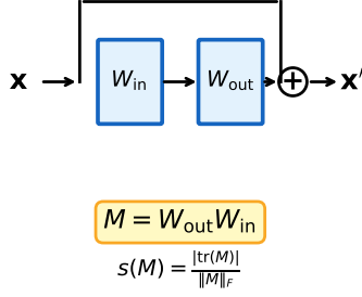
Figure 1: Training leaves traces in residual networks. (a) The residual branch product M = W_{\text{out}} W_{\text{in}} for a block with skip connection. (b) Diagonal dominance emerges only in trained residual networks: random initialization shows no structure (2% pair accuracy), trained ResNet shows strong diagonal (100%), and trained PlainNet without skip connections shows no signal (3%). (c) Lineage verification: descendants (fine-tuned, quantized, pruned, LoRA-merged) cluster near \mathcal{L} = 1 ; non-descendants (independent, distilled) remain near 0, enabling perfect separation.
