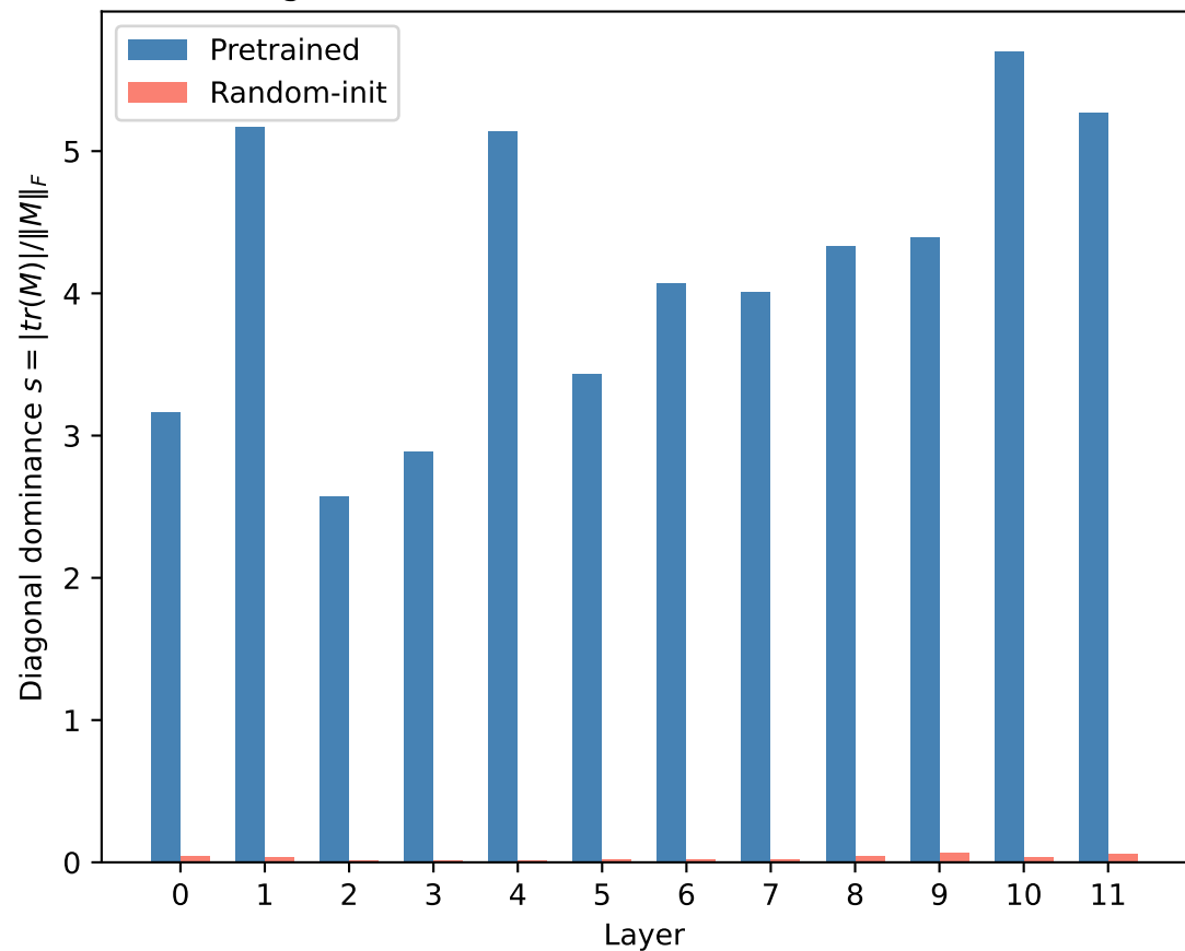
Diagonal Dominance: Pretrained vs Random-init
