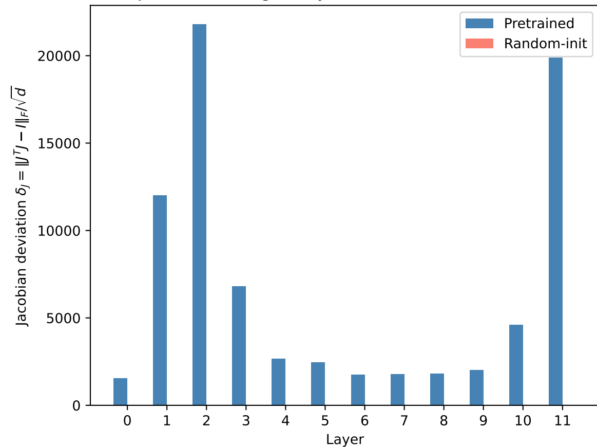
Jacobian Orthogonality: Pretrained vs Random-init
