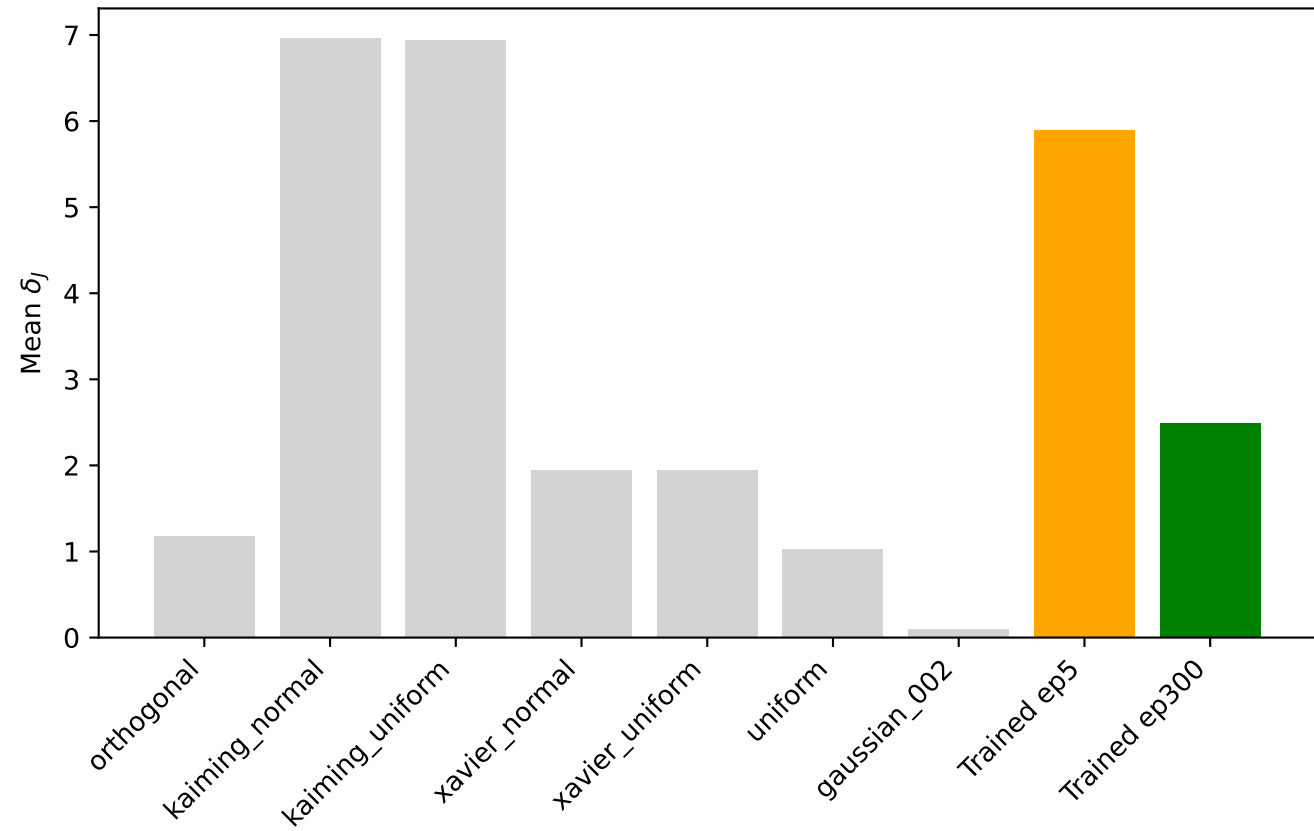
Jacobian Deviation by Condition
