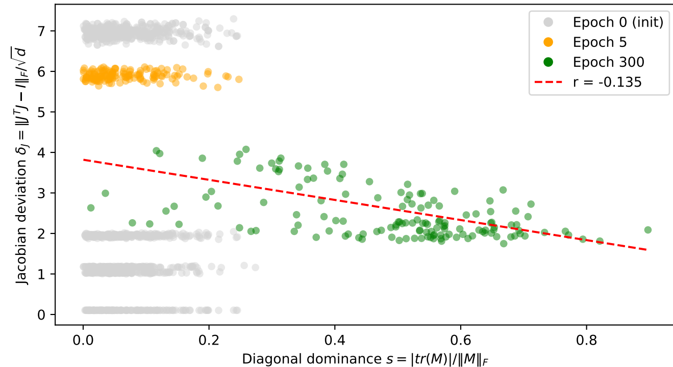
Jacobian Orthogonality vs Diagonal Dominance (all blocks, all conditions)
