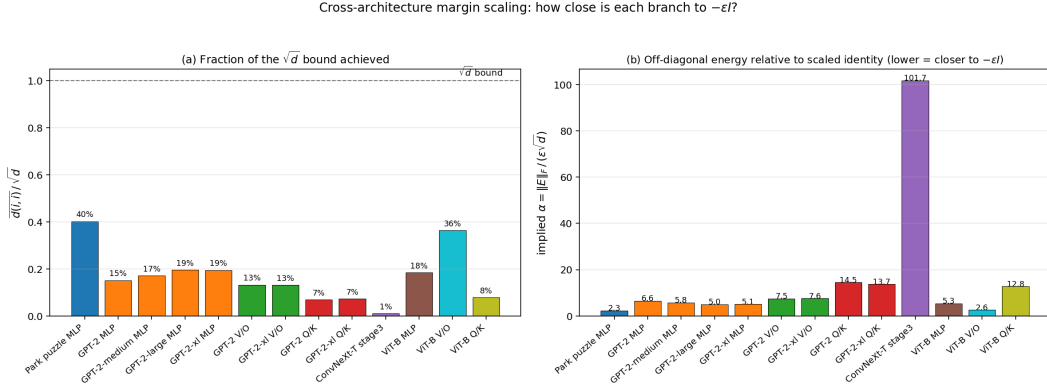
Figure 18. Cross-architecture margin scaling. (a) Fraction of the \sqrt{d} bound achieved by \overline{d(i, i)} for each architecture/path. (b) The implied off-diagonal-energy ratio \alpha . Three regimes emerge: high-isometry (Park puzzle MLP and ViT-B W_O W_V at 36–40% of the bound, \alpha \approx 2.5 ); mid-isometry (GPT-2 MLP family, ViT-B MLP at 15–19%); low-isometry (GPT-2 attention V/O and Q/K at 7–13%, with \alpha in [7, 14] ). ConvNeXt-T sits in an extreme regime ( \alpha \gtrsim 50 ) where the absolute d values are small but Hungarian pairing still recovers 100% via per-row rescue (Table 7).
