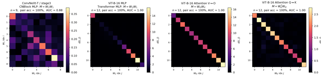
Figure 16. Diagonal-dominance matrices on modern vision architectures. (a) ConvNeXt-T stage 3 (9 CNBlocks) pairs at 100% via the MLP product W_2W_1 . (b) ViT-B/16 MLP (12 blocks) also pairs at 100% with AUC 1.000 and a strong depth-coded brightness gradient. (c) ViT-B/16 attention V \leftrightarrow O produces the single cleanest pair signal in this paper: sep = +4.84, AUC = 1.000, and 100% of correctly-paired products have negative trace — the full Proposition 1 prediction. (d) ViT-B/16 attention Q \leftrightarrow K also recovers 100% on a smaller absolute scale.
