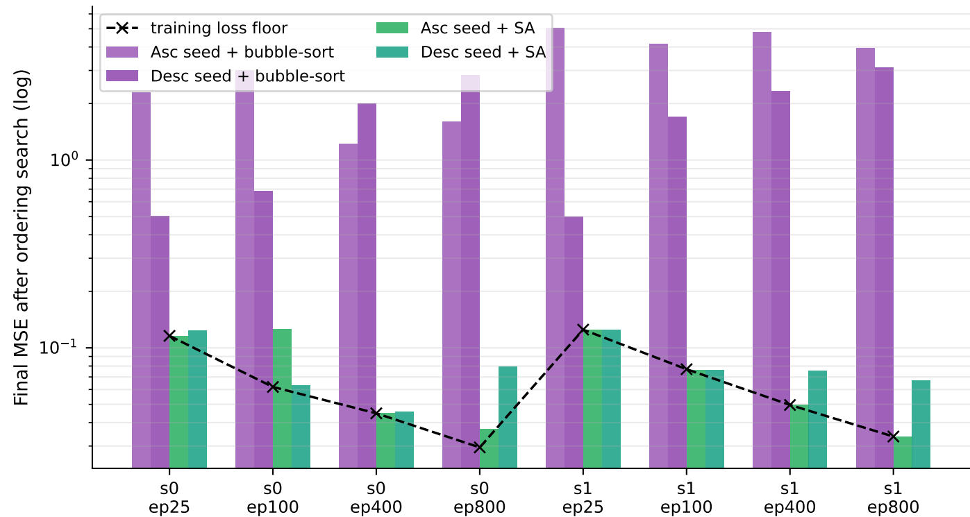
Bubble-sort never reaches the training-loss floor; SA reliably does
