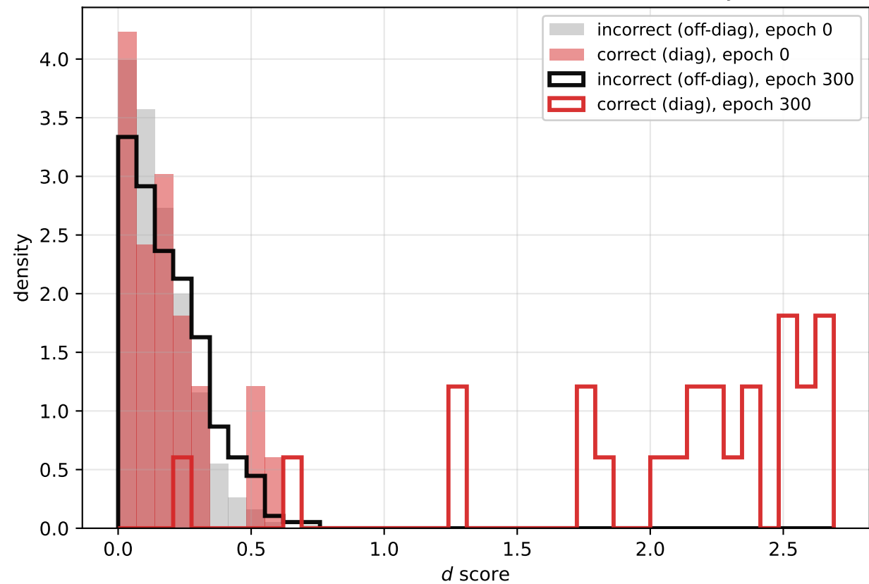
(c) Score distribution: untrained vs trained (overlay)
