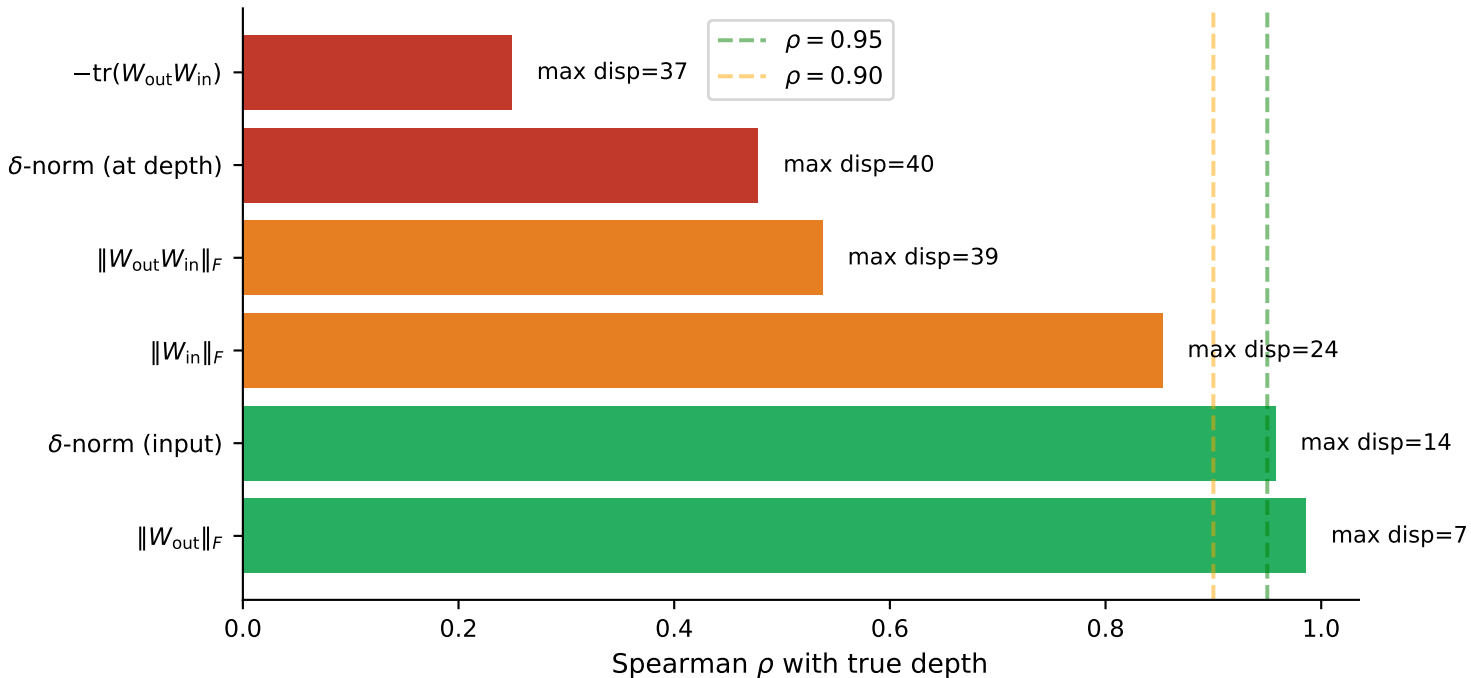
Seed-proxy rank correlation in Park's puzzle network ( \|W_{\text{out}}\|_F wins; \delta -norm second)
