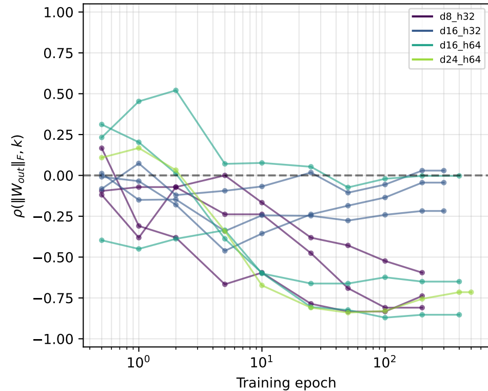
\rho(\|W_{out}\|_F, k)
