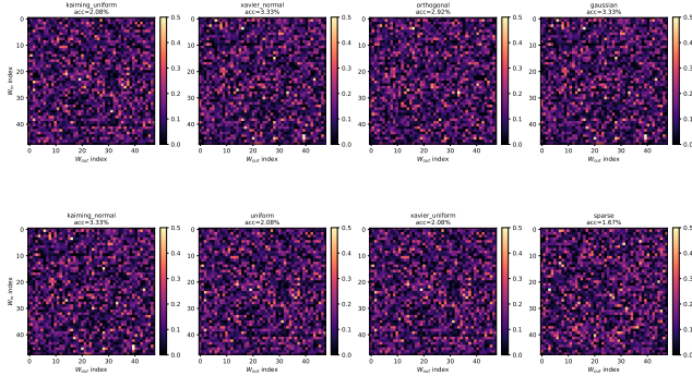
Figure 2: Initialization heatmaps. Score matrices s(i, j) at initialization under 8 schemes (orthogonal, Kaiming uniform/normal, Xavier uniform/normal, Gaussian \sigma=0.02 , uniform); pair accuracies span 1.67–3.33% (chance for 48 blocks is 2.1%). No scheme exhibits diagonal structure before training, including orthogonal init-which satisfies dynamical isometry by construction. Trained heatmaps reach 100% pair accuracy (Appendix A, Table 9). The fingerprint is therefore learned, not an initialization artifact.
