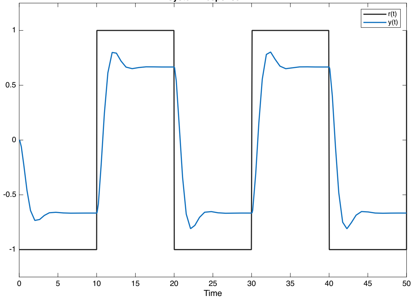
System Response K=2
