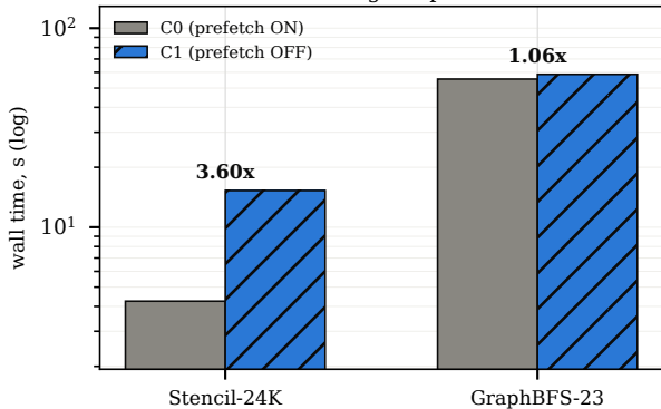
Cost: disabling the prefetcher
