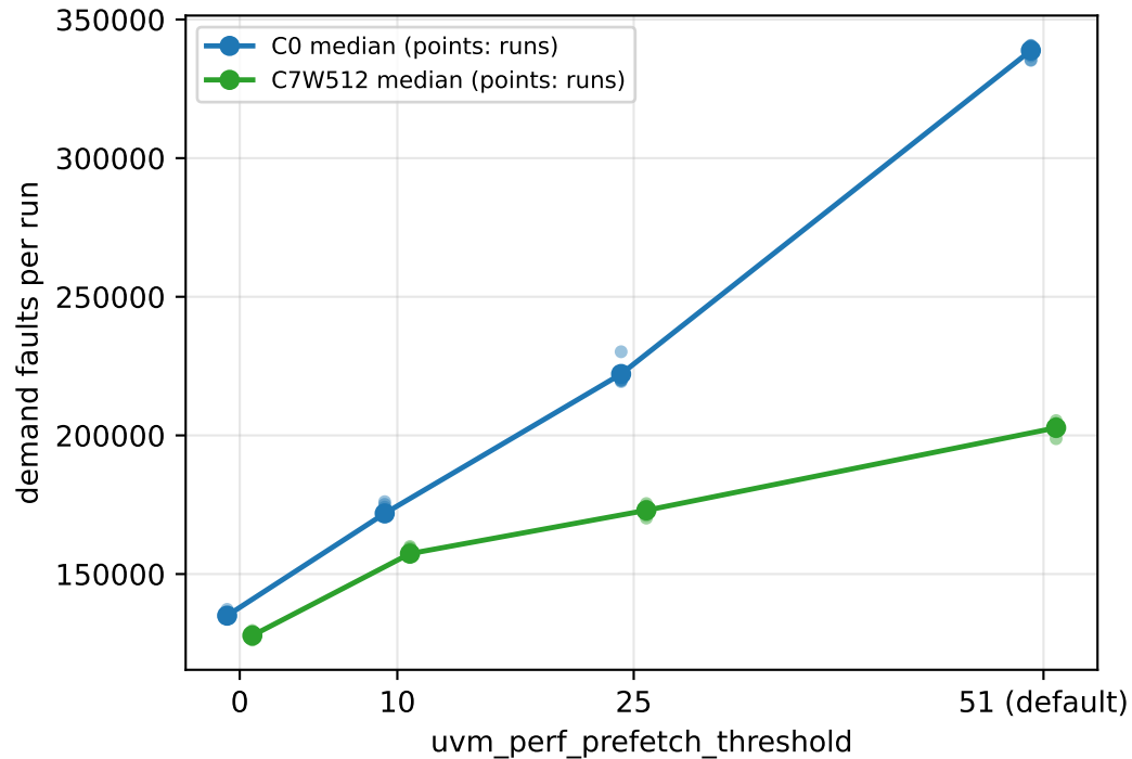
Gate E6: Stencil-24K, prefetcher on; C7W512 = cheap oracle + W=512 (n=10 per cell)
