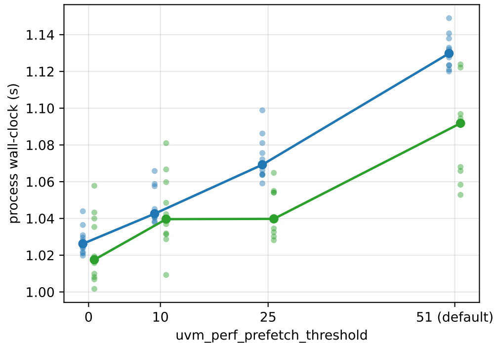
Gate E6: Stencil-24K, prefetcher on; C7W512 = cheap oracle + W=512 (n=10 per cell)
