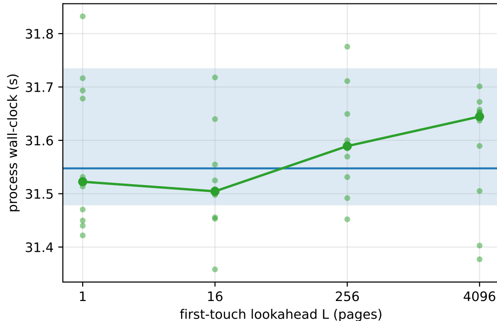
GraphBFS-23 (n=10 per cell)
