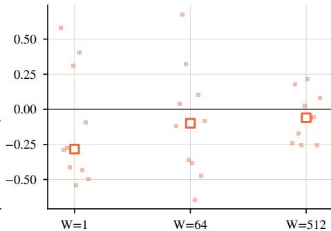
GraphBFS-23: staging width (cheap oracle, prefetcher on)
