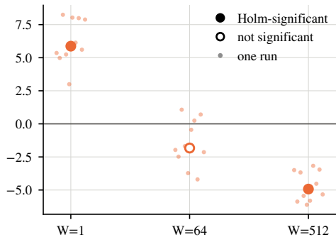
Stencil-24K: staging width (cheap oracle, prefetcher on)
