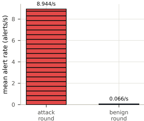
Linux ratio = 135.2x
