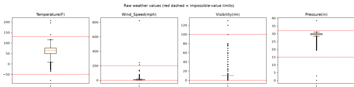
Figure 1. Weather values before cleaning. Box plots of the raw values; red dashed lines are the limits of Table 8.
