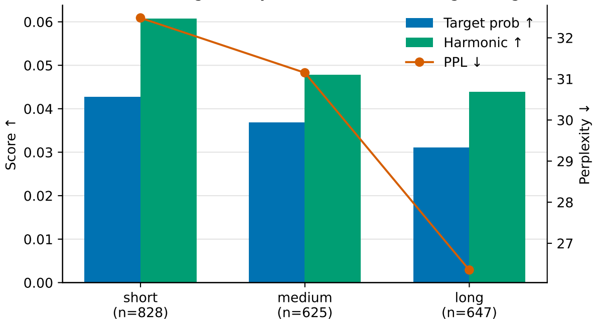
Sentence length analysis for the best steering setting
