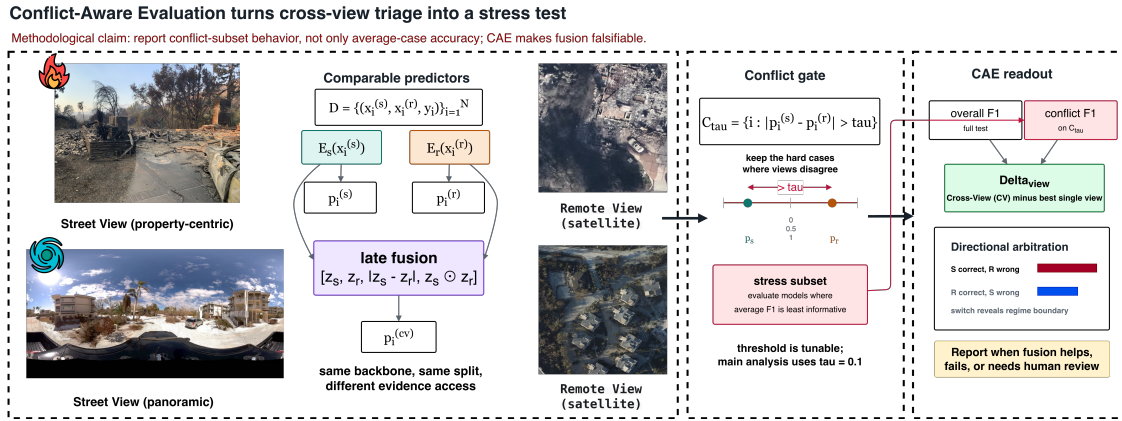
Figure 2: Conflict-Aware Evaluation (CAE) protocol. CAE isolates examples where street-only and remote-only predictors disagree, then reports whether cross-view fusion improves conflict-subset F1 over the stronger single-view baseline. Directional arbitration links model behavior to spatial observation regime.
