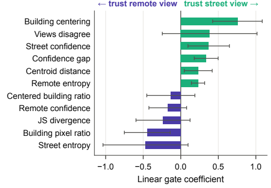
Figure 2: Coefficients of the two-expert (street vs. remote) linear gate on Eaton (mean \pm std over five seeds). Positive values shift trust toward the street view. Bars whose error bars cross zero do not have a stable sign across seeds.
