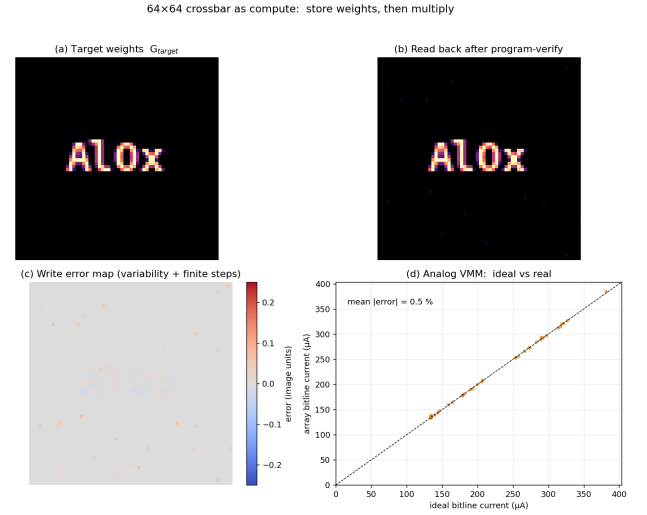
Fig. 10. Crossbar as compute. (a) Target weights (an image) and (b) the array read-back after program-verify. (c) Write-error map. (d) Analog MVM versus ideal, about 0.5 percent mean error.
