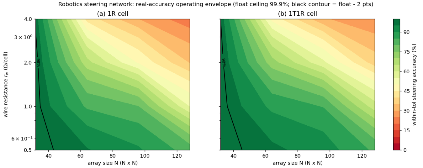
Fig. 15. Real task accuracy envelope for the PilotNet steering network mapped inference-only onto the calibrated \text{Ag}_2\text{O} crossbar. Accuracy is shown over array size N and wire resistance r_w for the passive 1R cell and the 1T1R cell. Both collapse monotonically with N and r_w ; the 1T1R cell is consistently more robust at large arrays because its access transistor relieves the IR drop. The black contour marks the float ceiling minus two points.
