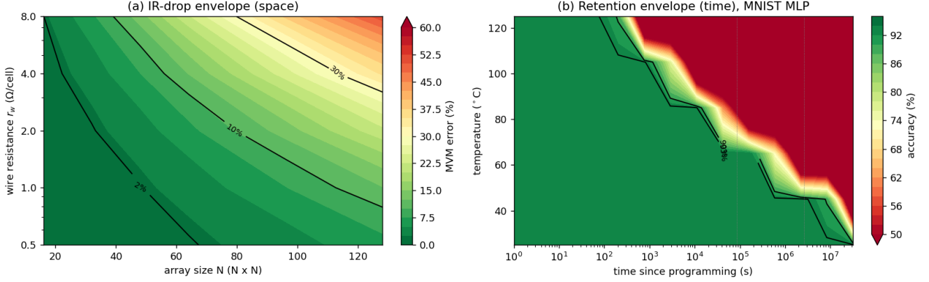
Fig. 12. Operating envelopes for the calibrated \text{Ag}_2\text{O} device. (a) IR-drop envelope: mean MVM error over array size and wire resistance, with 2/10/30 percent contours marking the naive-OK, training-recoverable, and IR-limited regions. (b) Retention envelope: accuracy of the trained MNIST MLP over time and temperature, with 90/93 percent contours giving the rewrite cadence.
