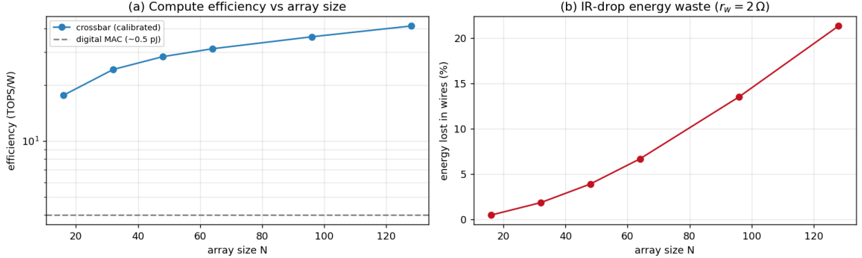
Fig. 13. Energy model for the calibrated device. (a) Compute efficiency (TOPS/W) versus array size, against a digital MAC reference. (b) Fraction of energy lost in the wires to IR drop, which grows with array size.
