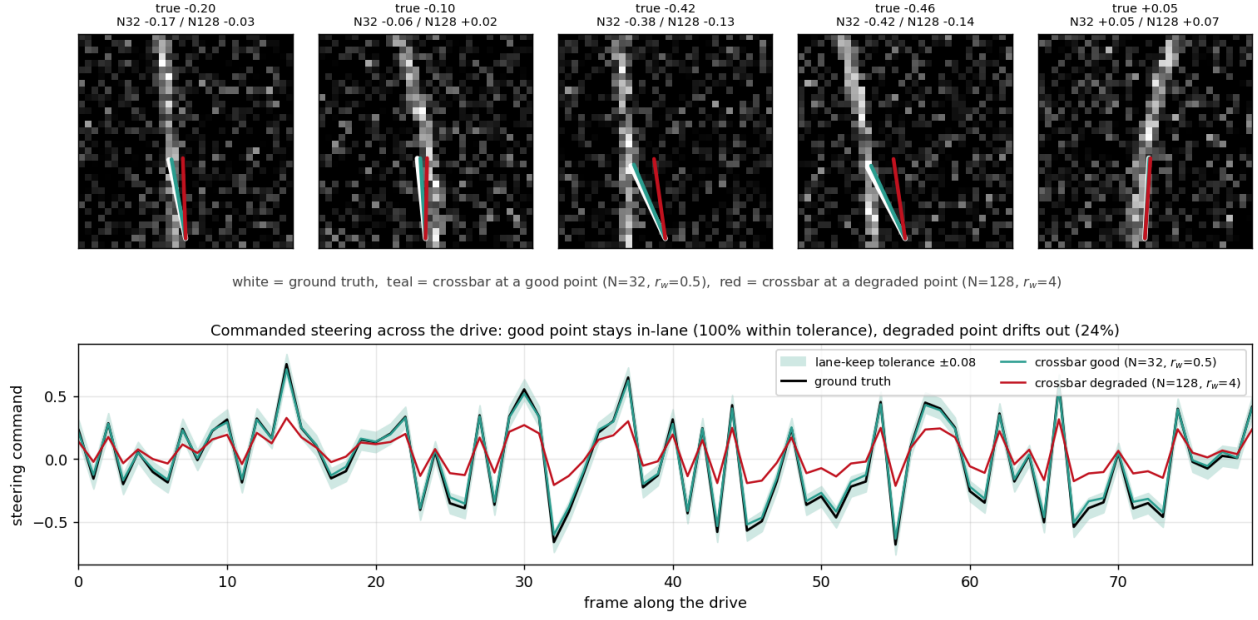
Fig. 14. The steering network running inference on the crossbar. Top: five road frames, each annotated with the ground-truth steering (white) and the crossbar-commanded steering at a good operating point (teal, N = 32, r_w = 0.5 ) and a degraded one (red, N = 128, r_w = 4 ). Bottom: the commanded steering across a drive. At the good point the crossbar tracks the reference inside the lane-keeping tolerance band (100 percent of frames in tolerance); at the degraded point it drifts out (24 percent), which would steer the vehicle out of its lane.
