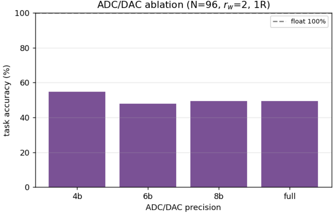
Fig. 17. ADC/DAC ablation at N = 96 , r_w = 2 , 1R cell. Real task accuracy is flat near 48 to 55 percent across 4, 6, 8, and full-precision converters, indicating that analog conductance and wire-resistance non-idealities, not converter bit depth, set accuracy in this IR-dominated regime.
