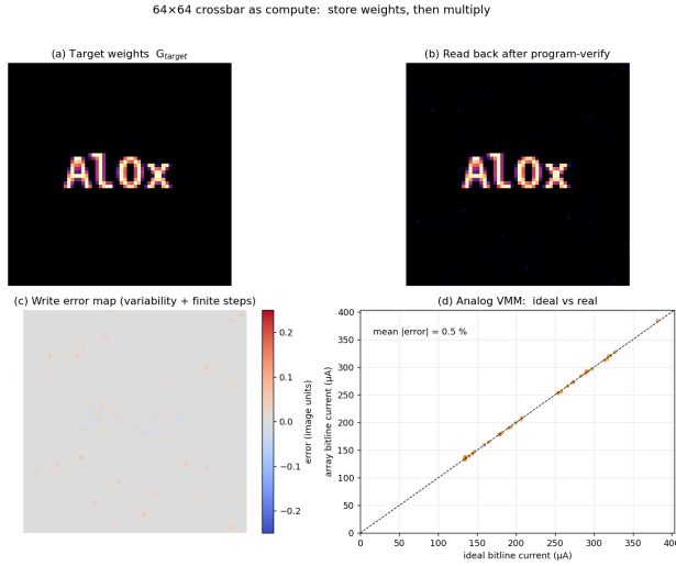
Fig. 18. Crossbar as compute. (a) Target weights (an image) and (b) the array read-back after program-verify. (c) Write-error map. (d) Analog MVM versus ideal, about 0.5 percent mean error.
