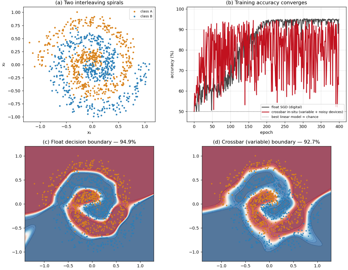
Fig. 9. In-situ learning on the crossbar (a representative seed; see text for seed statistics). (a) The two-spiral task. (b) Training accuracy converges for both floating-point SGD and the variable, noisy crossbar. (c, d) Learned decision boundaries; the crossbar closely matches floating point.
