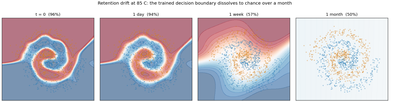
Fig. 11. The same trained network forgetting in time (frames left to right). As the conductances relax at 85 degrees Celsius, the decision boundary is intact at t = 0 and after one day, washes out by one week (57 percent), and is gone by one month (chance). No fixed set of weights can resist a time-varying decay.
