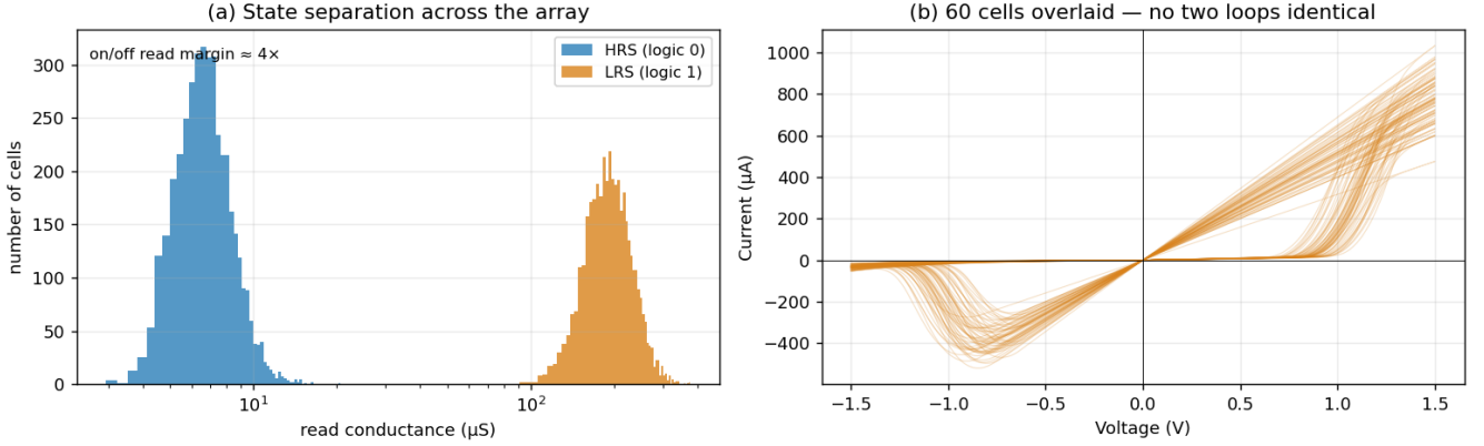
Fig. 4. 64×64 array (4096 cells). (a) HRS and LRS read-conductance distributions; the worst-case on/off margin (about 4x) is far smaller than the ratio of means (about 28x). (b) Current-voltage loops of 60 randomly chosen cells, showing device-to-device spread.
