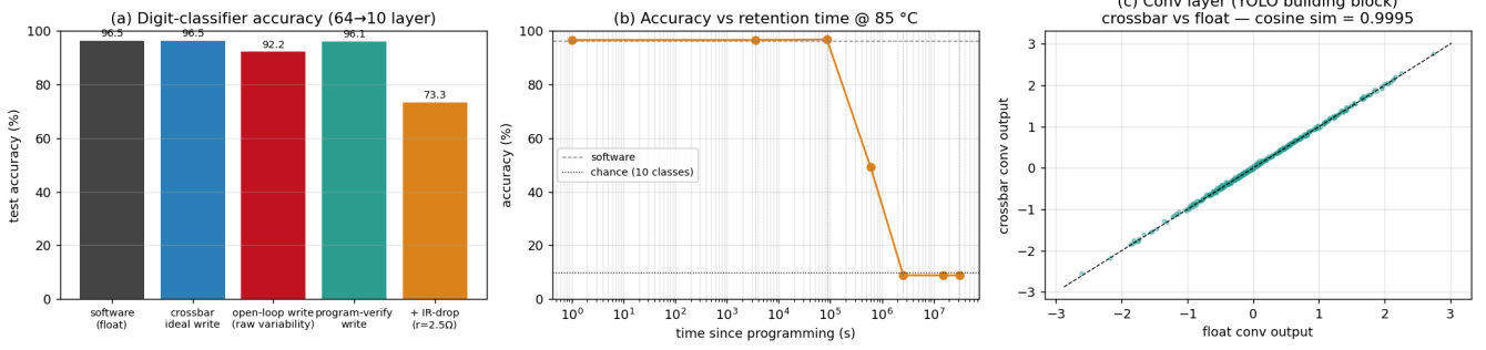
Fig. 5. Inference on the array. (a) Classifier accuracy across conditions: variability costs accuracy, program-verify recovers it, and IR drop then dominates. (b) Accuracy versus retention time at 85 degrees Celsius. (c) A convolutional layer (a YOLO building block) on the array reproduces the floating-point output with cosine similarity 0.999.
