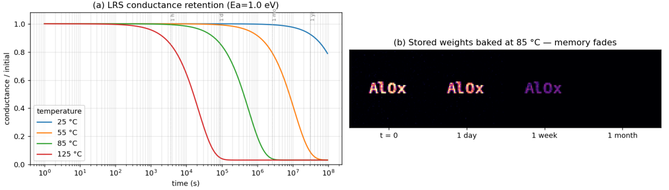
Fig. 8. Retention. (a) Normalized LRS conductance versus time at four temperatures; each temperature shifts the decay by roughly a decade. (b) A stored weight pattern baked at 85 degrees Celsius fades from sharp to gone over a month.
