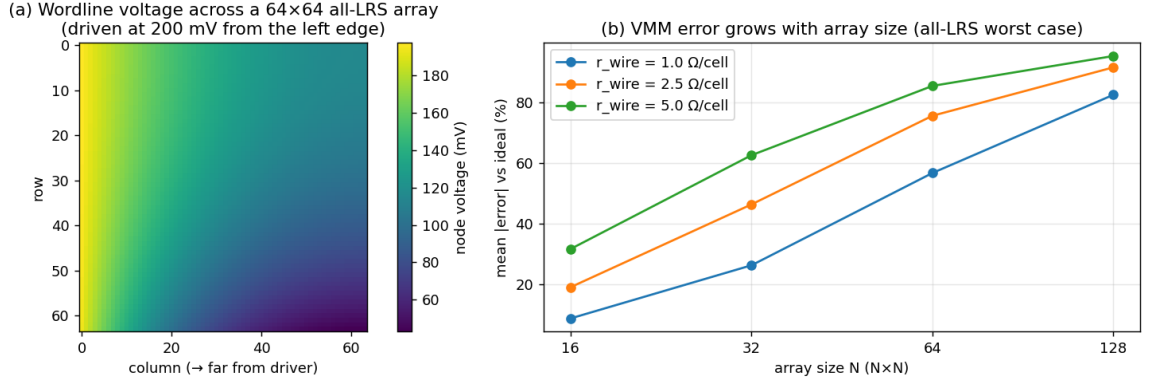
Fig. 7. Wire IR drop from the full nodal solve. (a) Wordline voltage across a 64x64 all-LRS array driven at 200 mV; the voltage droops toward the far corner. (b) Mean MVM error versus array size for three wire resistances (worst case).
