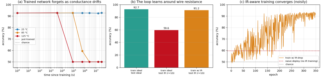
Fig. 10. Two interactions of non-idealities with a trained network. (a) Retention drift after training: accuracy holds for about a day at 85 degrees Celsius, then dissolves to chance by one month. (b) IR drop: naive deployment under wire resistance collapses accuracy, but training with IR drop in the loop recovers it. (c) The IR-aware training converges (with a pulse-size decay schedule).
