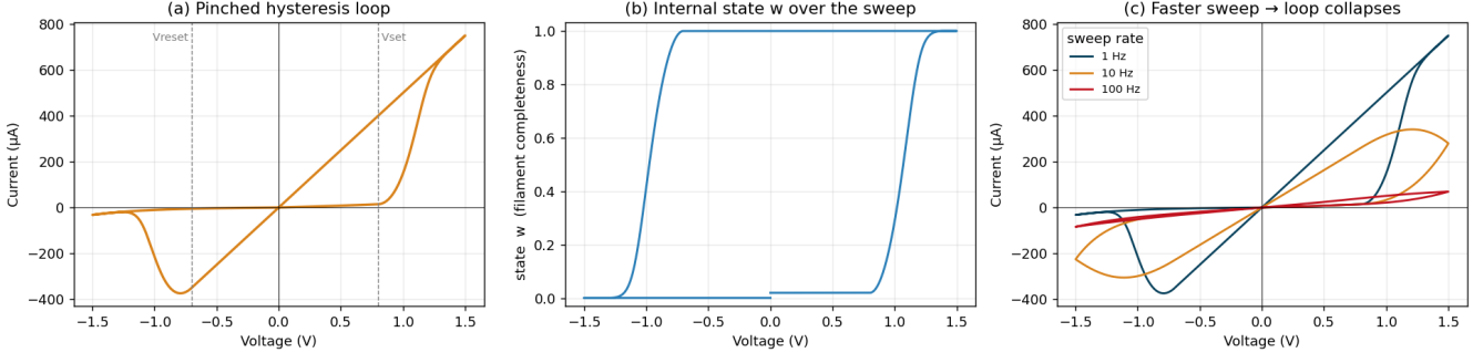
Fig. 3. Single AlO x cell. (a) Pinched hysteresis loop. (b) State variable w over the sweep, showing threshold-gated SET and RESET. (c) The loop area collapses monotonically as sweep frequency increases and the state can no longer fully switch.
