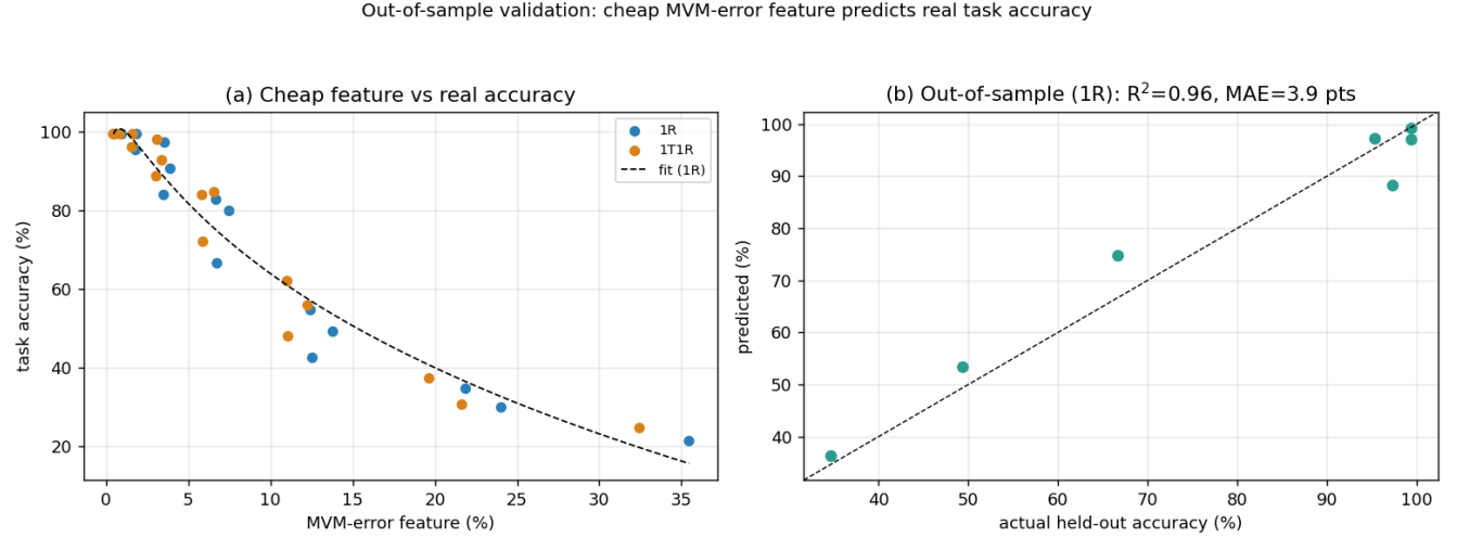
Fig. 16. Out-of-sample validation of the cheap MVM-error feature against real task accuracy. (a) Real accuracy versus the feature for all grid configurations, with the degree-2 fit. (b) Held-out predictions versus actual accuracy lie on the diagonal: R^2 = 0.96 , MAE 3.9 points, so the feature predicts the real task accuracy of configurations it never saw, making the envelope predictive.
