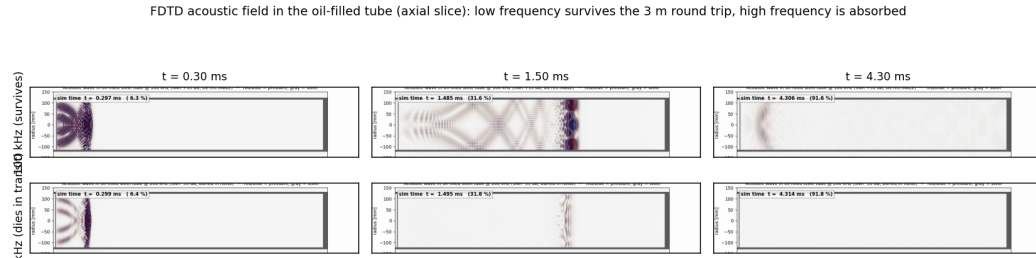
Figure 3: FDTD acoustic field on an axial slice. Top: at 100 kHz the pulse travels the full 3 m, reflects, and returns (echo present near the near end at 4.30 ms). Bottom: at 200 kHz the pulse is absorbed before completing the round trip, so no echo returns. The contrast is the f^2 absorption cliff made visible. The full three-panel movies for each frequency are released at https://github.com/rayjyotir5/pmut-tube-echo/tree/main/media (files 100khz.mp4, 135khz.mp4, 200khz.mp4).
