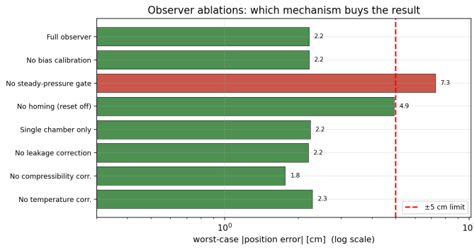
Fig. 14. Observer ablations (worst case over a temperature/seed subset, log scale). Removing the steady-pressure gate or the homing reset is what breaks the result; the physical corrections are minor.
