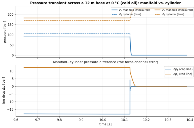
Fig. 19. Hopsan pressure transient across a 12 m hose at 0 °C. Top: measured manifold pressures (solid) sit \sim 12 –18 bar off the true cylinder pressures (dashed)—a force read directly from the manifold inherits this gap. Bottom: the line drop \Delta p for each chamber, steady between events and spiking at the reversal near 10.1 s.
