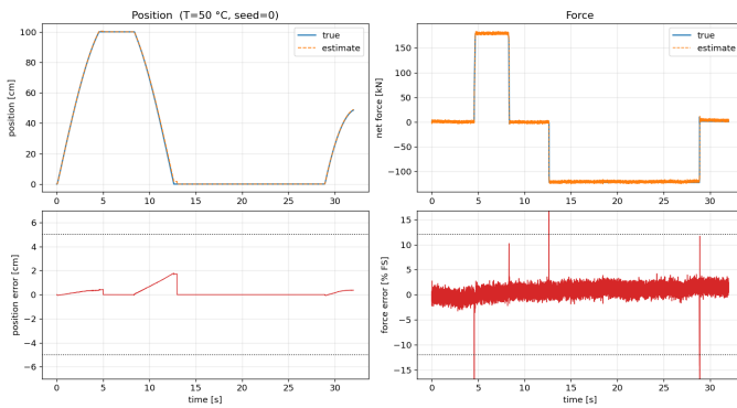
Fig. 10. Representative run at 50 °C. Left: true vs estimated position and the error against the \pm 5 cm band (note the bias drift growing between homing events and resetting at each seat). Right: net force and its error against the \pm 12\% FS band; the brief spikes are the flow-reversal transients a delayed transducer cannot track. Dotted lines are the limits.
