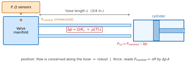
Fig. 2. Manifold-located sensing. The transducers tap the valve block; a hose of length L carries oil to the cylinder, dropping pressure by \Delta p . Position is unaffected (flow is conserved along the hose) but the force read-out inherits the full \Delta p A offset, which grows with length and with colder, more viscous oil.
