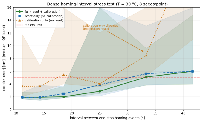
Fig. 15. Dense homing-interval stress test (median, inter-quartile band; 8 seeds). Full (●) and reset-only (■) nearly coincide and hold \pm 5 cm out to \sim 30 s; calibration-only (▲, no position reset) is worse everywhere and diverges. The homing reset, not the bias calibration, is what bounds the error.
