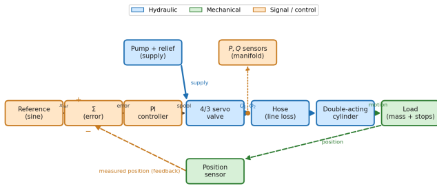
Fig. 3. Block schematic of the Hopsan plant: a PI position controller drives a 4/3 servo valve feeding a double-acting cylinder against a mass / end-stop load, a relief-limited pump supplies pressure, and a position sensor closes the loop. Blue is the hydraulic domain, green mechanical, orange signal/control. The detailed model as built in Hopsan is shown in Fig. 5.
