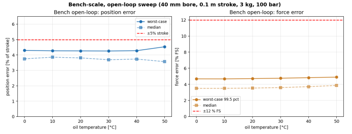
Fig. 21. Bench-scale, open-loop sweep (40 mm bore, 0.1 m stroke, 3 kg, 100 bar; no position controller). Worst-case position stays at \sim 4.3 % of stroke and force below 5 % FS across 0–50 °C, once the homing reset identifies the seated stop from direction of travel rather than from chamber pressure.
