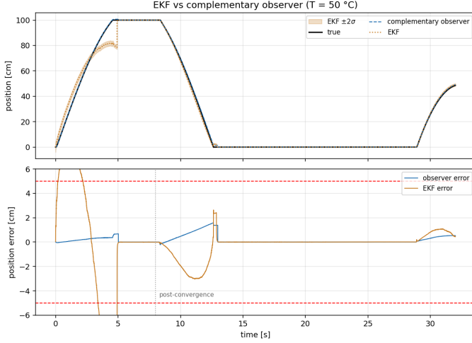
Fig. 22. EKF vs complementary observer on one run (50 °C). Top: position, with the EKF \pm 2\sigma band. Bottom: errors against the \pm 5 cm band. The EKF lags the first ramp until its first homing and has larger transients; the observer stays tighter throughout.
