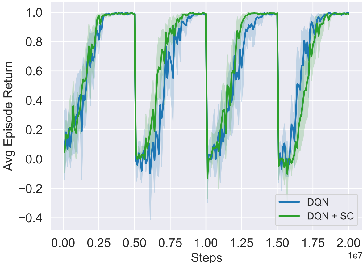
3D Four Rooms environment
