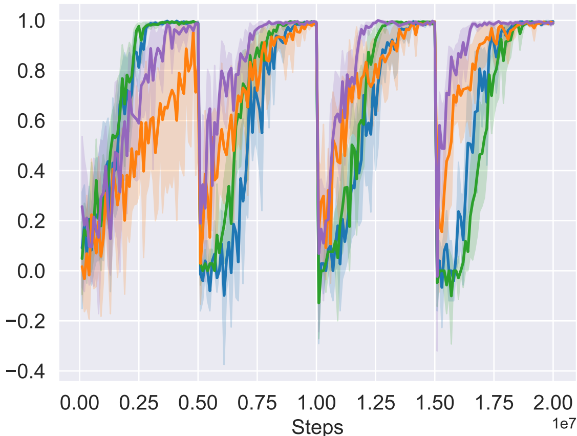
Avg Episode Returns
