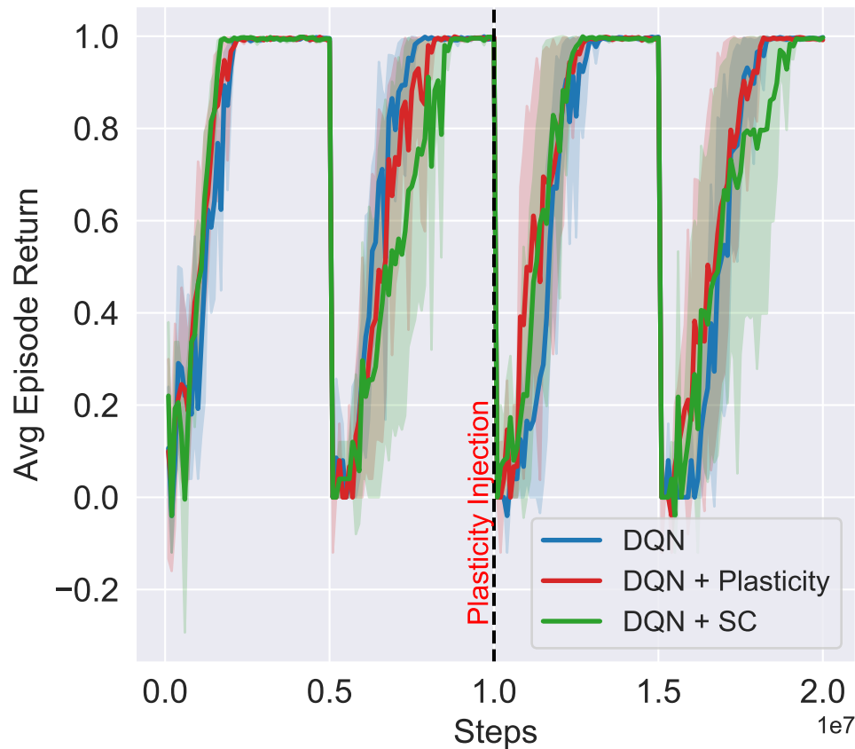
Consolidating Q-values shows limited benefits beyond first task
