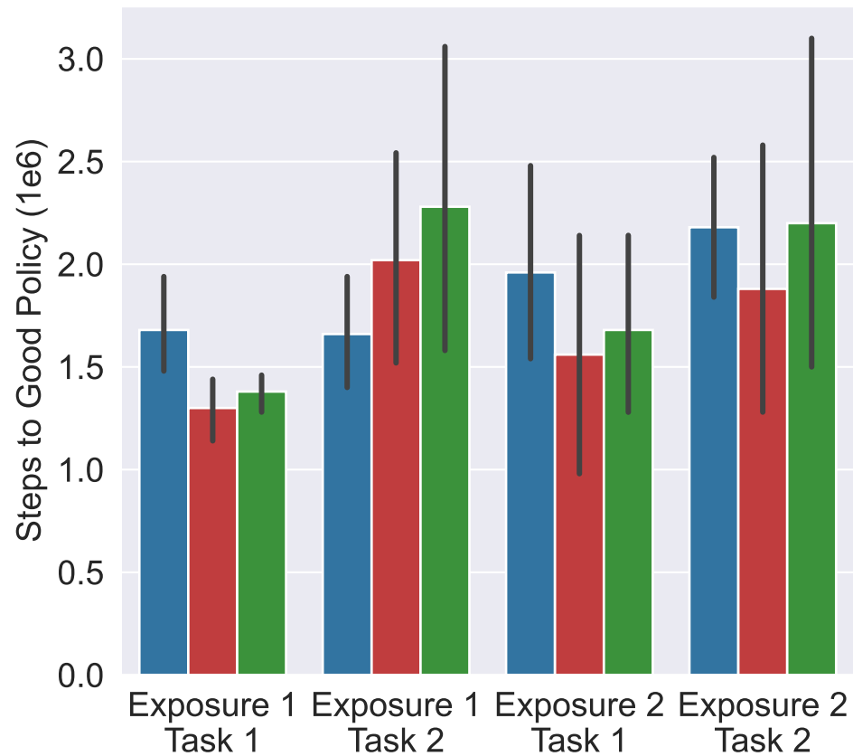
Consolidating Q-values shows limited benefits beyond first task
