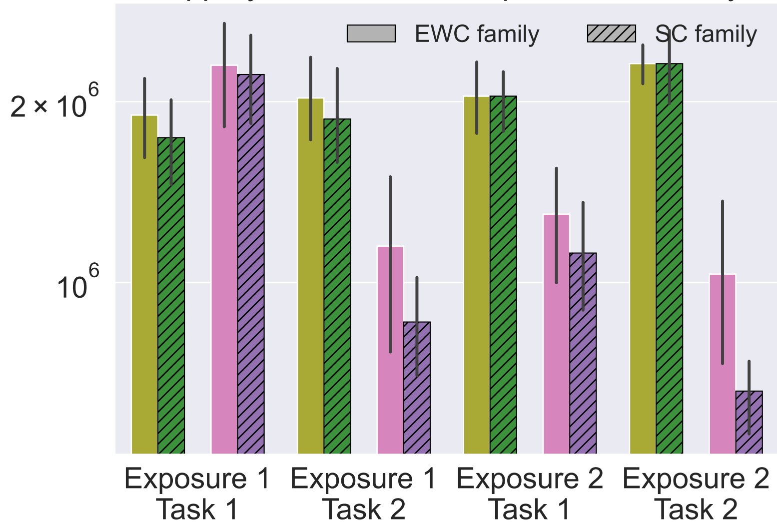
Slippery Four Rooms: Steps to Good Policy
