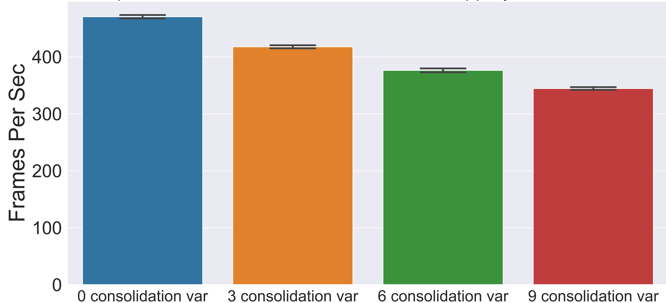
Computational Cost of SF Consolidation for Slippery Four Rooms Env
