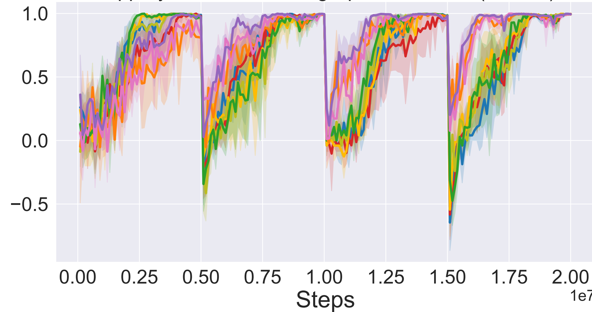
Slippery Four Rooms: Avg Episode Return (Severe)
