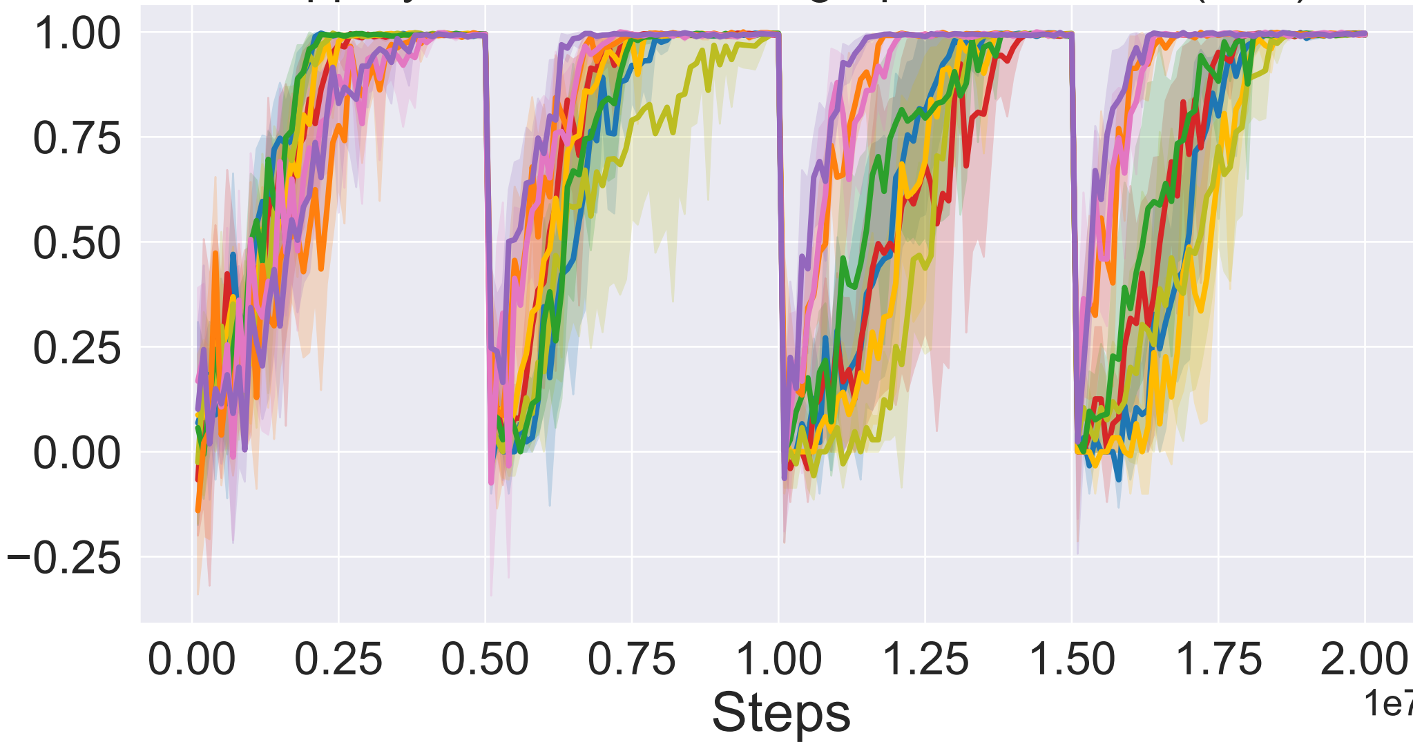
Slippery Four Roomsh: Avg Episode Return (Mild)
