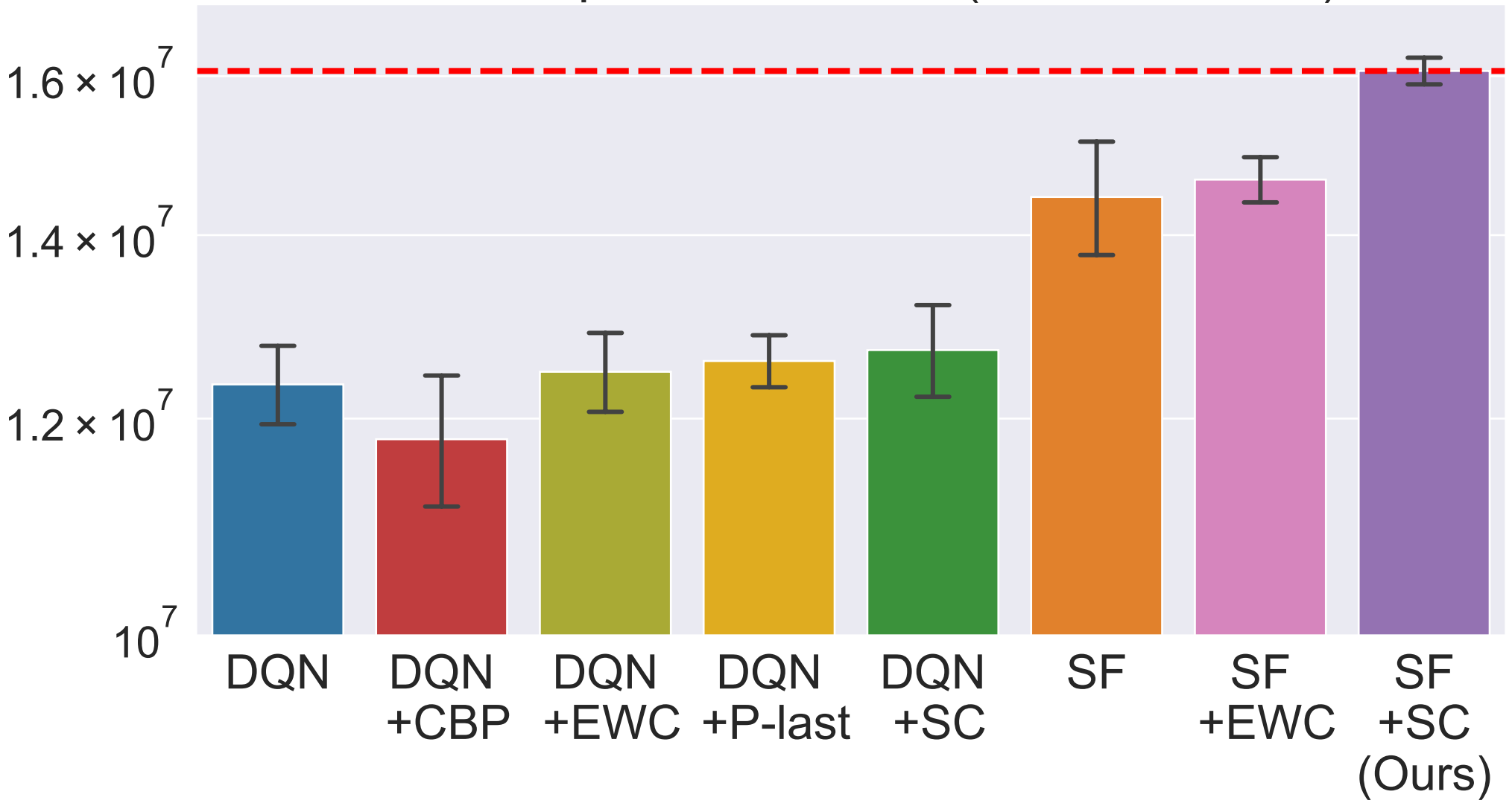
AUC of Episode Rewards (Severe - 100%)
