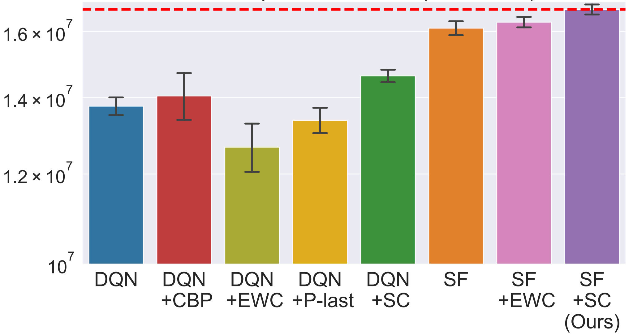
AUC of Episode Rewards (Mild - 25%)
