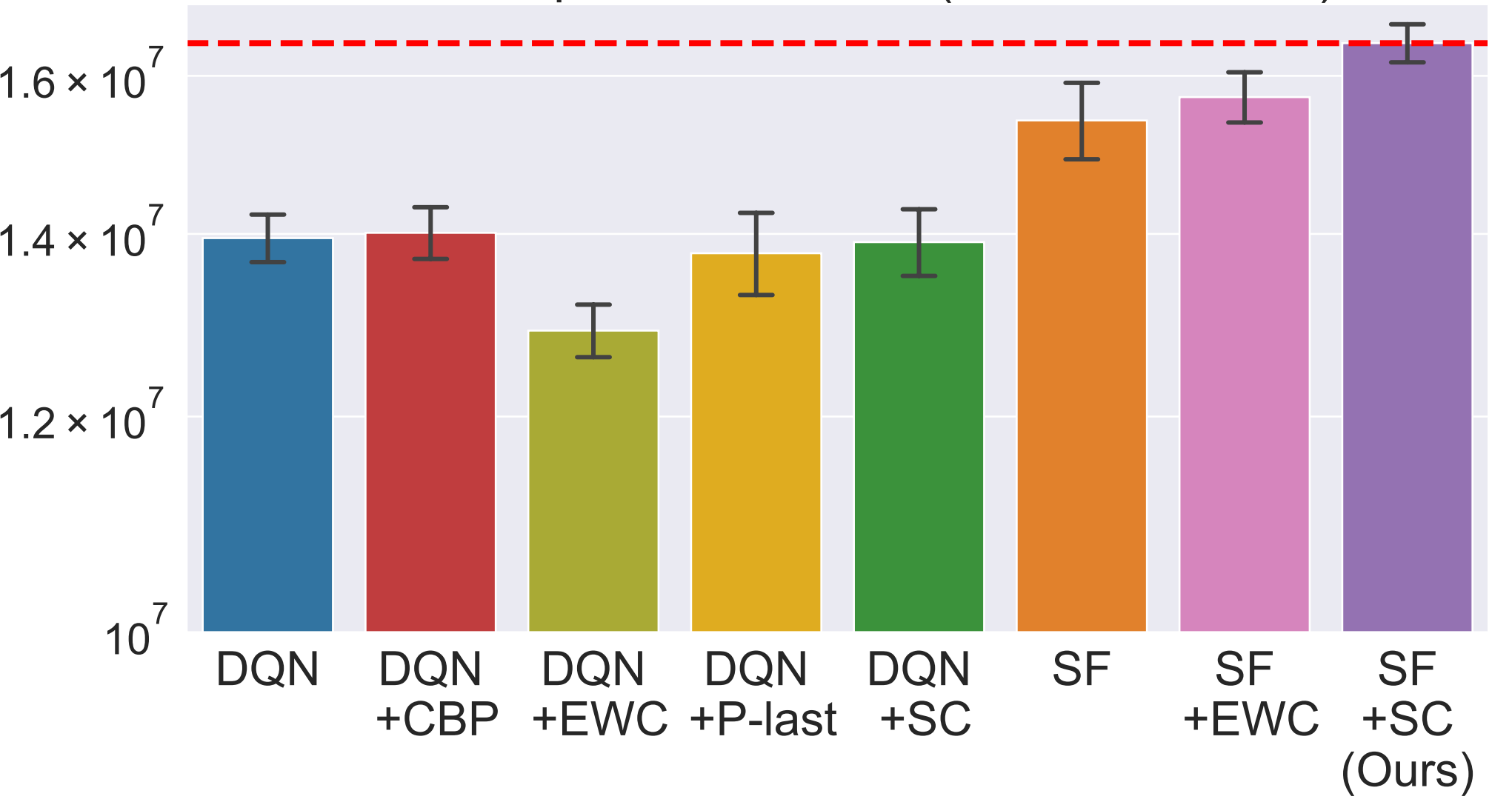
AUC of Episode Rewards (Moderate - 50%)
