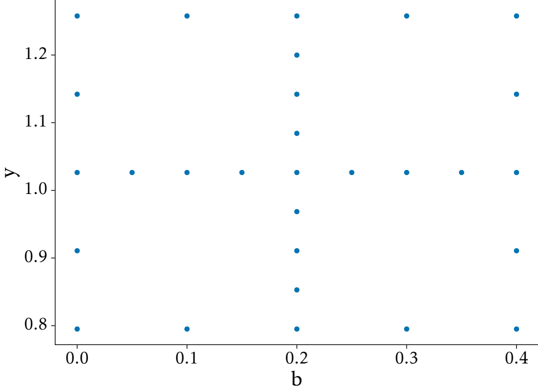
Figure 14: Smolyak Sparse Grid Points
