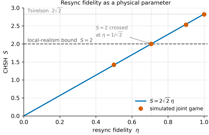
Figure 6. The resync-fidelity law S = 2\sqrt{2}\eta . Degrading the conditional update to fidelity \eta scales the CHSH value linearly; the simulated joint game (points) tracks the law, crosses the local-realism bound S = 2 exactly at \eta = 1/\sqrt{2} , and reaches the Tsirelson value 2\sqrt{2} at \eta = 1 . The fidelity \eta is thereby a measurable physical parameter, not an interpretive gloss.
