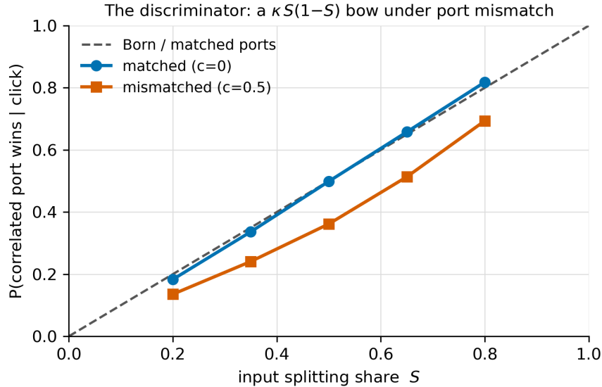
Figure 7. The tabletop discriminator. Conditional probability that the correlated port registers, versus the input splitting share S . Matched ports ( c = 0 ) track the Born diagonal; deliberately mismatched within-port noise correlation ( c = 0.5 ) produces the predicted \kappa S(1 - S) bow, suppressing the internally-correlated port. Any nonzero curvature beyond calibrated efficiency effects discriminates against the linear-POVM structure of standard quantum mechanics.
