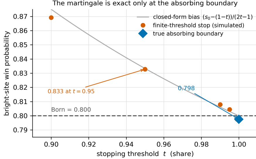
Figure 3. The martingale reproduces Born only at the true absorbing boundary. Stopping the game at a finite share and taking the argmax biases the winner probability upward by the closed-form amount (s_0 - (1-t))/(2t-1) (grey curve); the two-site 2:1 configuration gives 0.833 at threshold t = 0.95 , converging to Born (0.80) as t \rightarrow 1 , and the true absorbing boundary (last survivor) reproduces Born to the Monte-Carlo floor. This is the artifact identified in review and its resolution.
