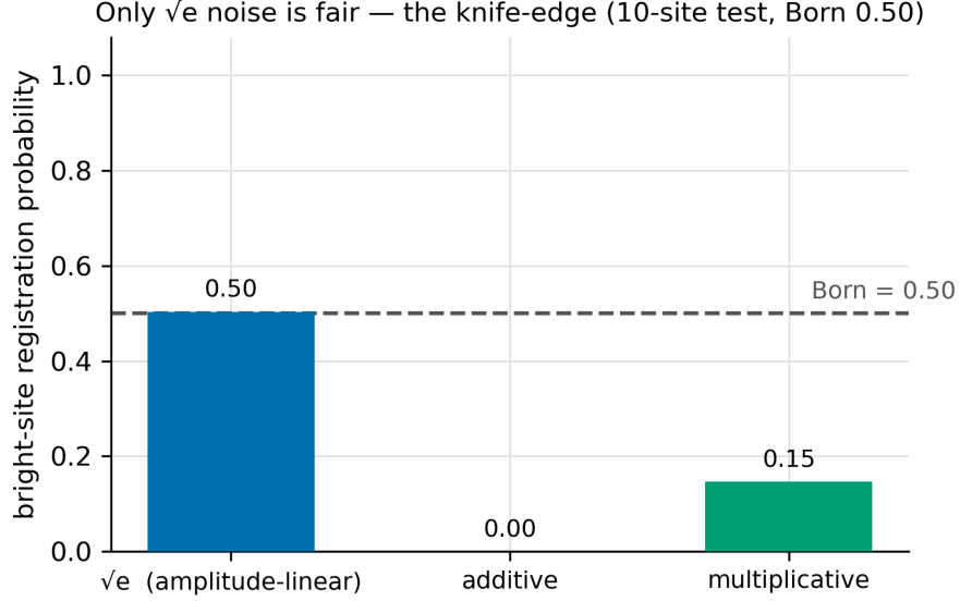
Figure 2. The knife-edge (10-site test configuration, Born weight of the bright site 0.50). Only amplitude-linear ( \sqrt{e} ) noise is fair; state-independent (additive) noise drives the bright site toward certainty, and multiplicative noise over-equalizes. Corrected absorbing-boundary simulation.
