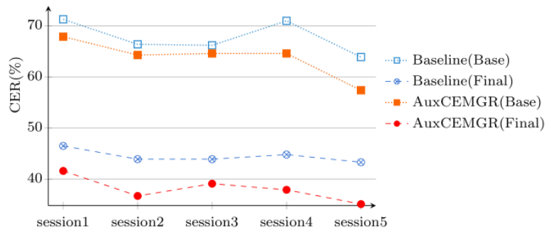
Fig. 11. CER of the four models on each session.
